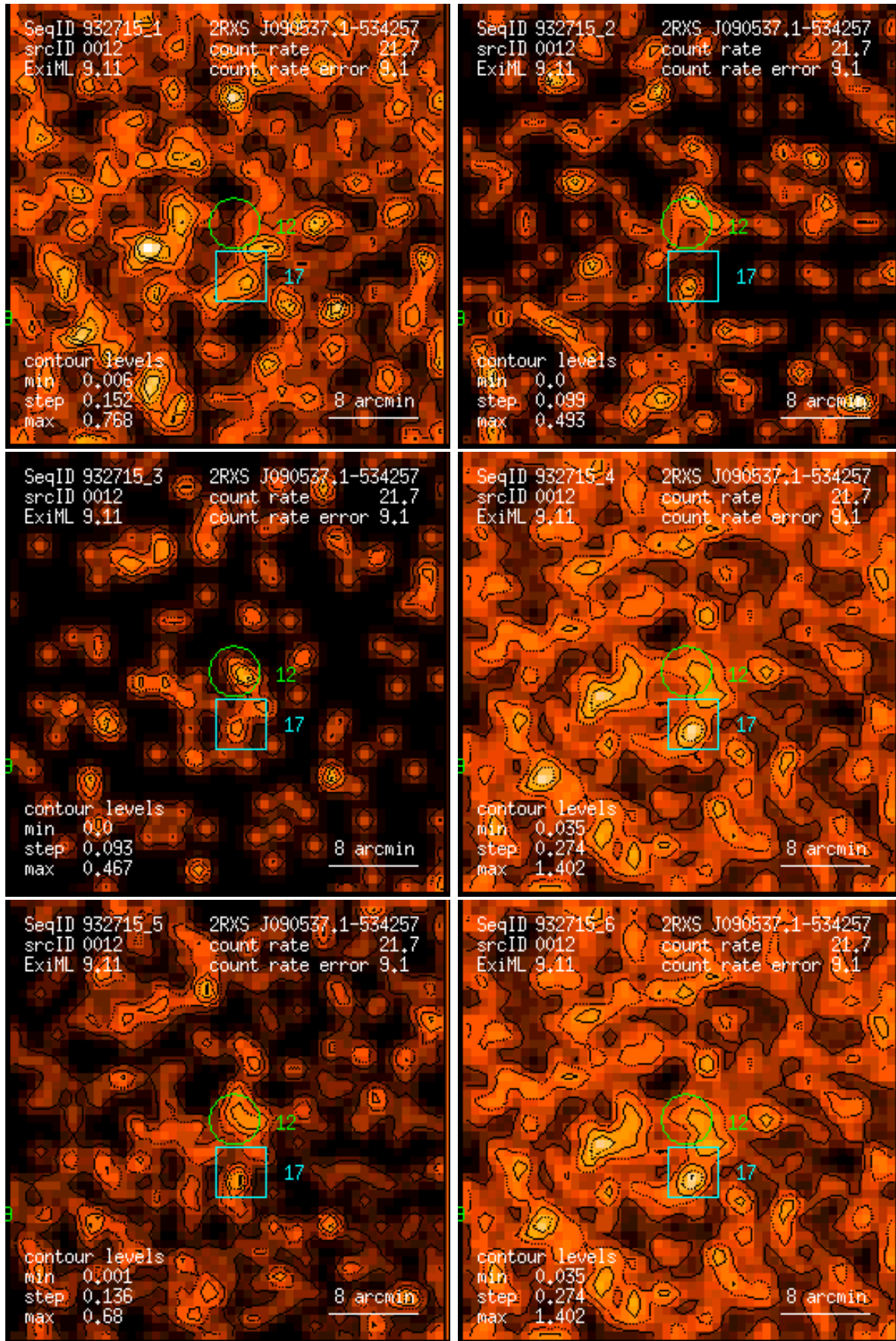
Figure 12: RASS 932715: detection 0012: band rate images, Gaussian filter: (1) PSPC channels 11 – 41, (2) 52 – 90, (3) 91 – 201, (4) 11 – 235, (5) 52 – 201, (6) 11 – 201. Broad band rates in counts/ks. Band rate contour levels in counts/ks/arcmin 2 .
