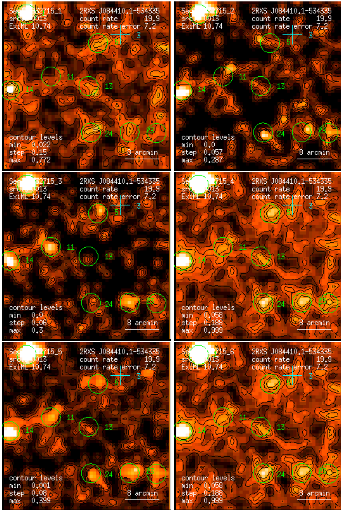
Figure 13: RASS 932715: detection 0013: band rate images, Gaussian filter: (1) PSPC channels 11 – 41, (2) 52 – 90, (3) 91 – 201, (4) 11 – 235, (5) 52 – 201, (6) 11 – 201. Broad band rates in counts/ks. Band rate contour levels in counts/ks/arcmin 2 .
