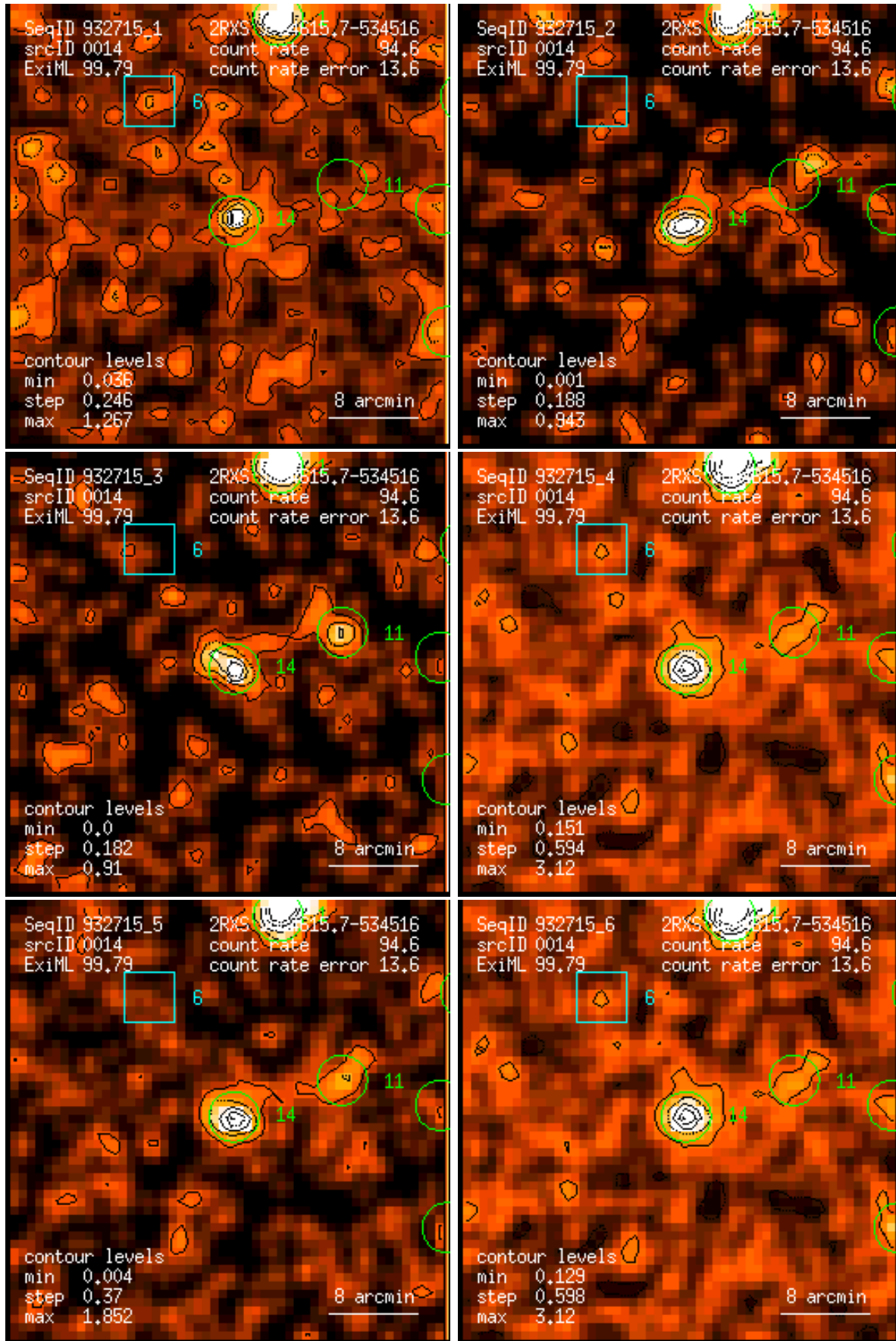
Figure 14: RASS 932715: detection 0014: band rate images, Gaussian filter: (1) PSPC channels 11 – 41, (2) 52 – 90, (3) 91 – 201, (4) 11 – 235, (5) 52 – 201, (6) 11 – 201. Broad band rates in counts/ks. Band rate contour levels in counts/ks/arcmin 2 .
