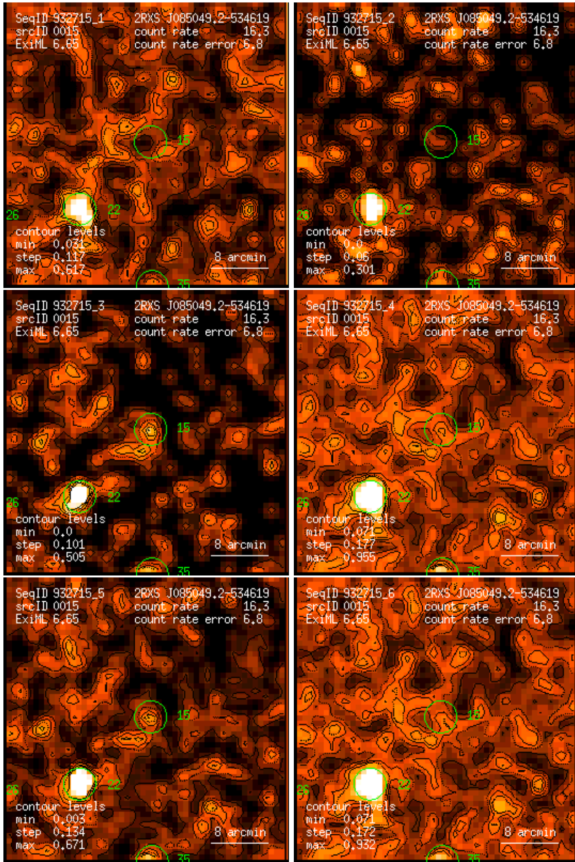
Figure 15: RASS 932715: detection 0015: band rate images, Gaussian filter: (1) PSPC channels 11 – 41, (2) 52 – 90, (3) 91 – 201, (4) 11 – 235, (5) 52 – 201, (6) 11 – 201. Broad band rates in counts/ks. Band rate contour levels in counts/ks/arcmin 2 .
