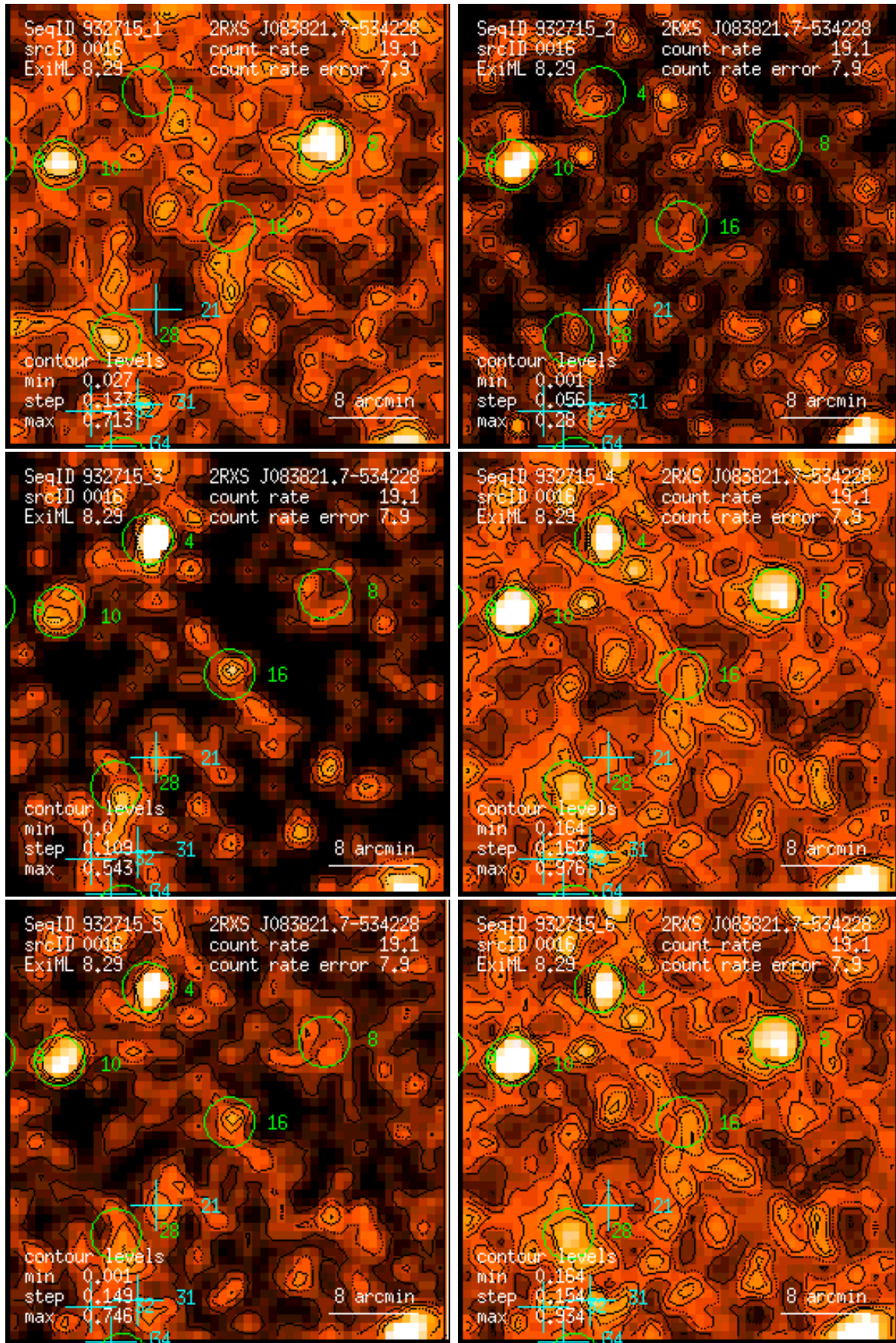
Figure 16: RASS 932715: detection 0016: band rate images, Gaussian filter: (1) PSPC channels 11 – 41, (2) 52 – 90, (3) 91 – 201, (4) 11 – 235, (5) 52 – 201, (6) 11 – 201. Broad band rates in counts/ks. Band rate contour levels in counts/ks/arcmin 2 .
