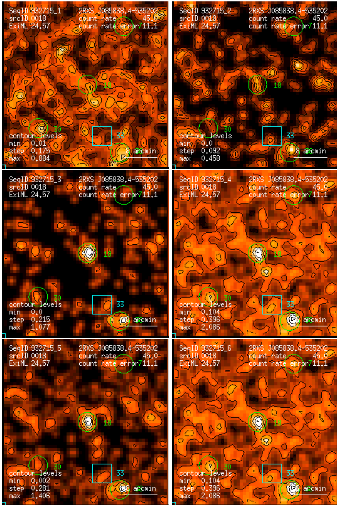
Figure 18: RASS 932715: detection 0018: band rate images, Gaussian filter: (1) PSPC channels 11 – 41, (2) 52 – 90, (3) 91 – 201, (4) 11 – 235, (5) 52 – 201, (6) 11 – 201. Broad band rates in counts/ks. Band rate contour levels in counts/ks/arcmin 2 .
