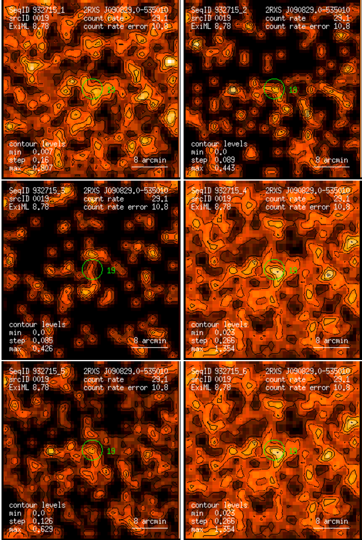
Figure 19: RASS 932715: detection 0019: band rate images, Gaussian filter: (1) PSPC channels 11 – 41, (2) 52 – 90, (3) 91 – 201, (4) 11 – 235, (5) 52 – 201, (6) 11 – 201. Broad band rates in counts/ks. Band rate contour levels in counts/ks/arcmin 2 .
