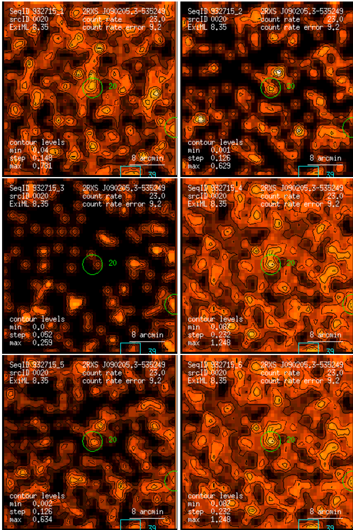
Figure 20: RASS 932715: detection 0020: band rate images, Gaussian filter: (1) PSPC channels 11 – 41, (2) 52 – 90, (3) 91 – 201, (4) 11 – 235, (5) 52 – 201, (6) 11 – 201. Broad band rates in counts/ks. Band rate contour levels in counts/ks/arcmin 2 .
