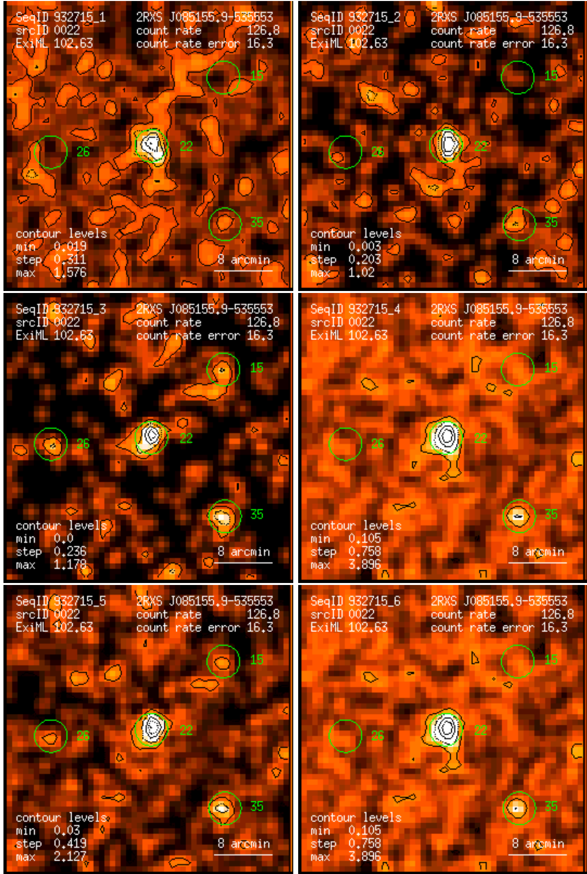
Figure 22: RASS 932715: detection 0022: band rate images, Gaussian filter: (1) PSPC channels 11 – 41, (2) 52 – 90, (3) 91 – 201, (4) 11 – 235, (5) 52 – 201, (6) 11 – 201. Broad band rates in counts/ks. Band rate contour levels in counts/ks/arcmin 2 .
