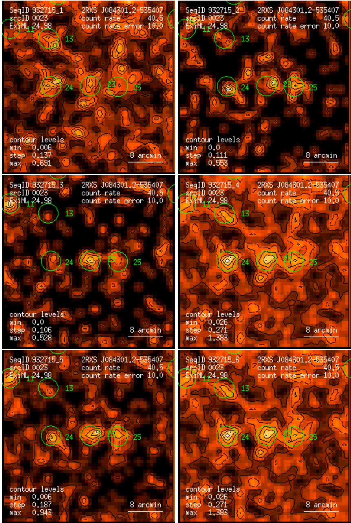
Figure 23: RASS 932715: detection 0023: band rate images, Gaussian filter: (1) PSPC channels 11 – 41, (2) 52 – 90, (3) 91 – 201, (4) 11 – 235, (5) 52 – 201, (6) 11 – 201. Broad band rates in counts/ks. Band rate contour levels in counts/ks/arcmin 2 .
