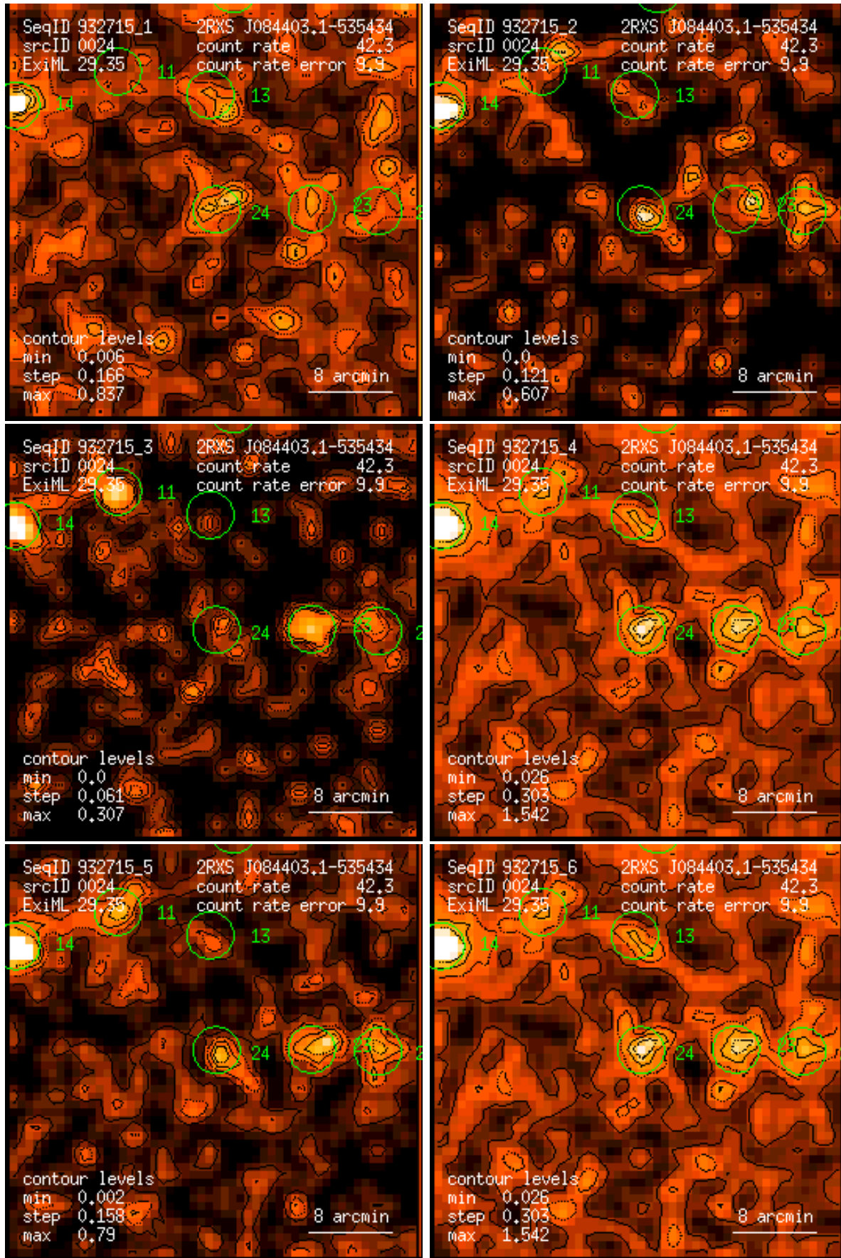
Figure 24: RASS 932715: detection 0024: band rate images, Gaussian filter: (1) PSPC channels 11 – 41, (2) 52 – 90, (3) 91 – 201, (4) 11 – 235, (5) 52 – 201, (6) 11 – 201. Broad band rates in counts/ks. Band rate contour levels in counts/ks/arcmin 2 .
