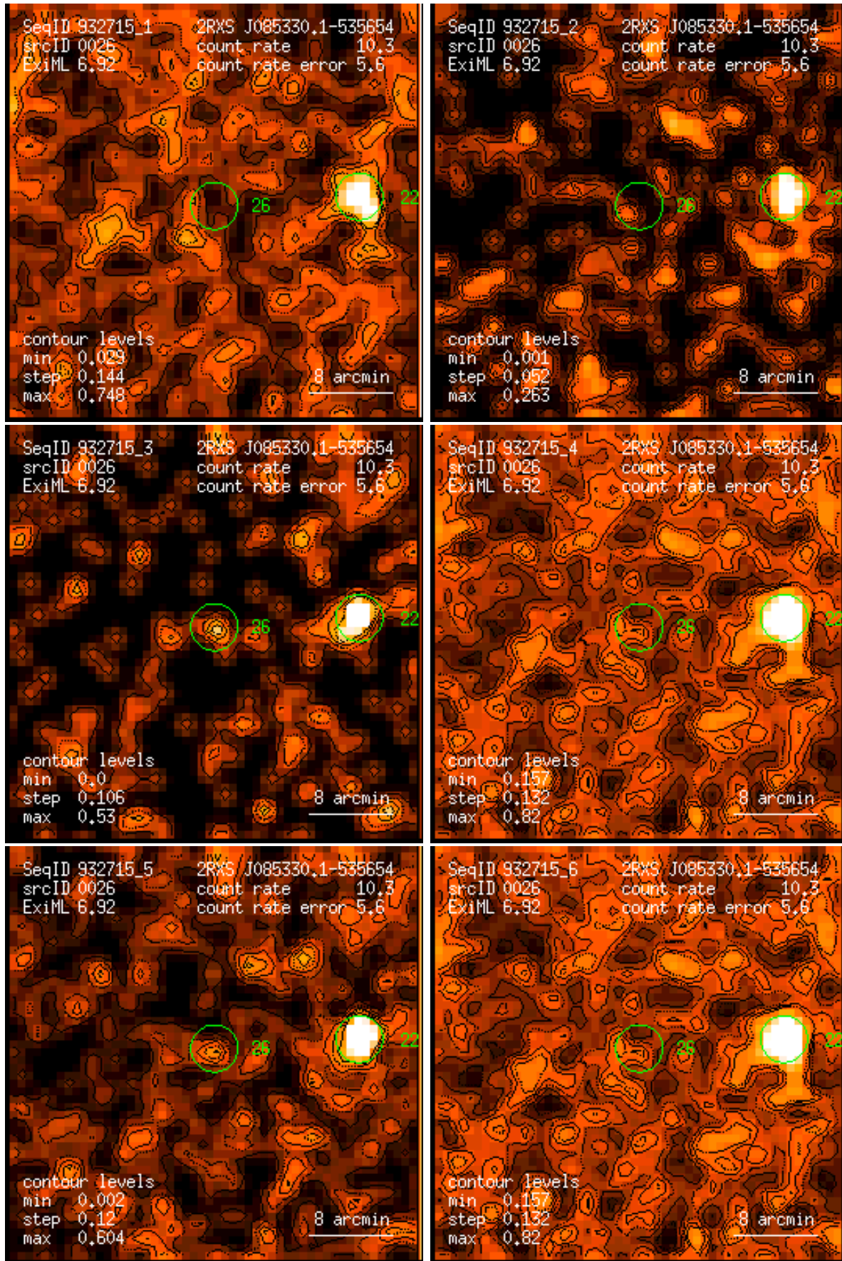
Figure 26: RASS 932715: detection 0026: band rate images, Gaussian filter: (1) PSPC channels 11 – 41, (2) 52 – 90, (3) 91 – 201, (4) 11 – 235, (5) 52 – 201, (6) 11 – 201. Broad band rates in counts/ks. Band rate contour levels in counts/ks/arcmin 2 .
