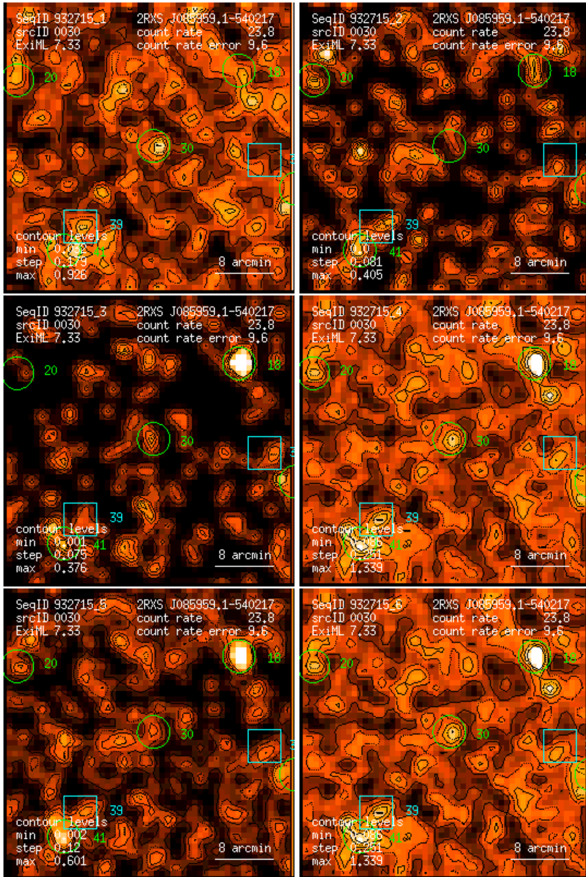
Figure 30: RASS 932715: detection 0030: band rate images, Gaussian filter: (1) PSPC channels 11 – 41, (2) 52 – 90, (3) 91 – 201, (4) 11 – 235, (5) 52 – 201, (6) 11 – 201. Broad band rates in counts/ks. Band rate contour levels in counts/ks/arcmin 2 .
