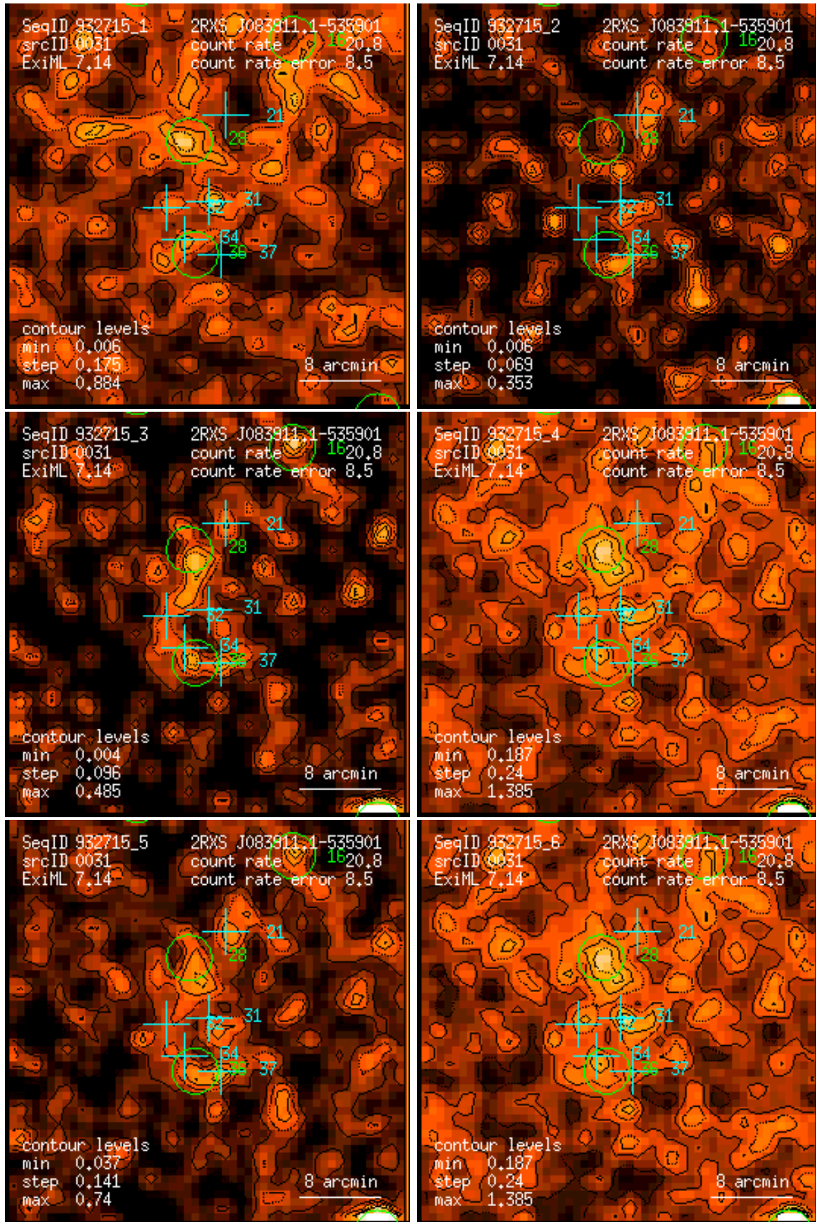
Figure 31: RASS 932715: detection 0031: band rate images, Gaussian filter: (1) PSPC channels 11 – 41, (2) 52 – 90, (3) 91 – 201, (4) 11 – 235, (5) 52 – 201, (6) 11 – 201. Broad band rates in counts/ks. Band rate contour levels in counts/ks/arcmin 2 .
