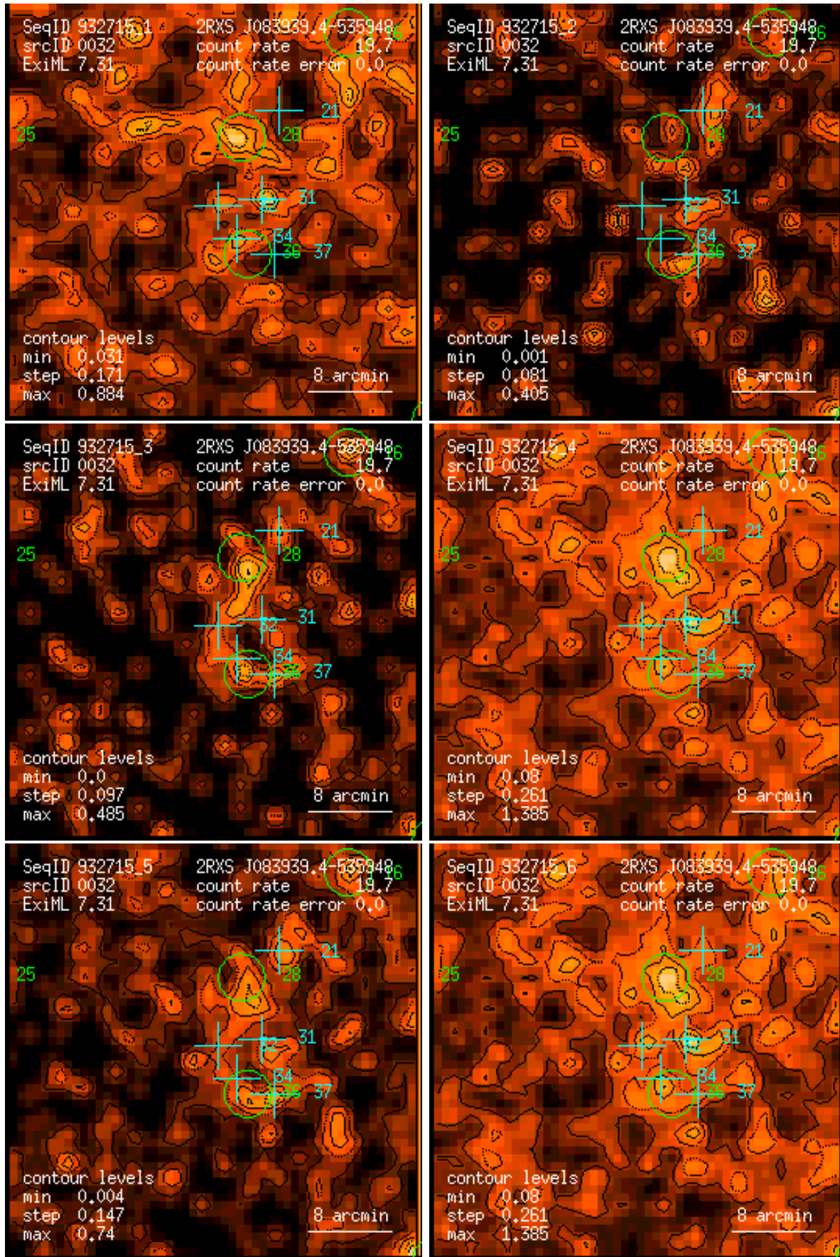
Figure 32: RASS 932715: detection 0032: band rate images, Gaussian filter: (1) PSPC channels 11 – 41, (2) 52 – 90, (3) 91 – 201, (4) 11 – 235, (5) 52 – 201, (6) 11 – 201. Broad band rates in counts/ks. Band rate contour levels in counts/ks/arcmin 2 .
