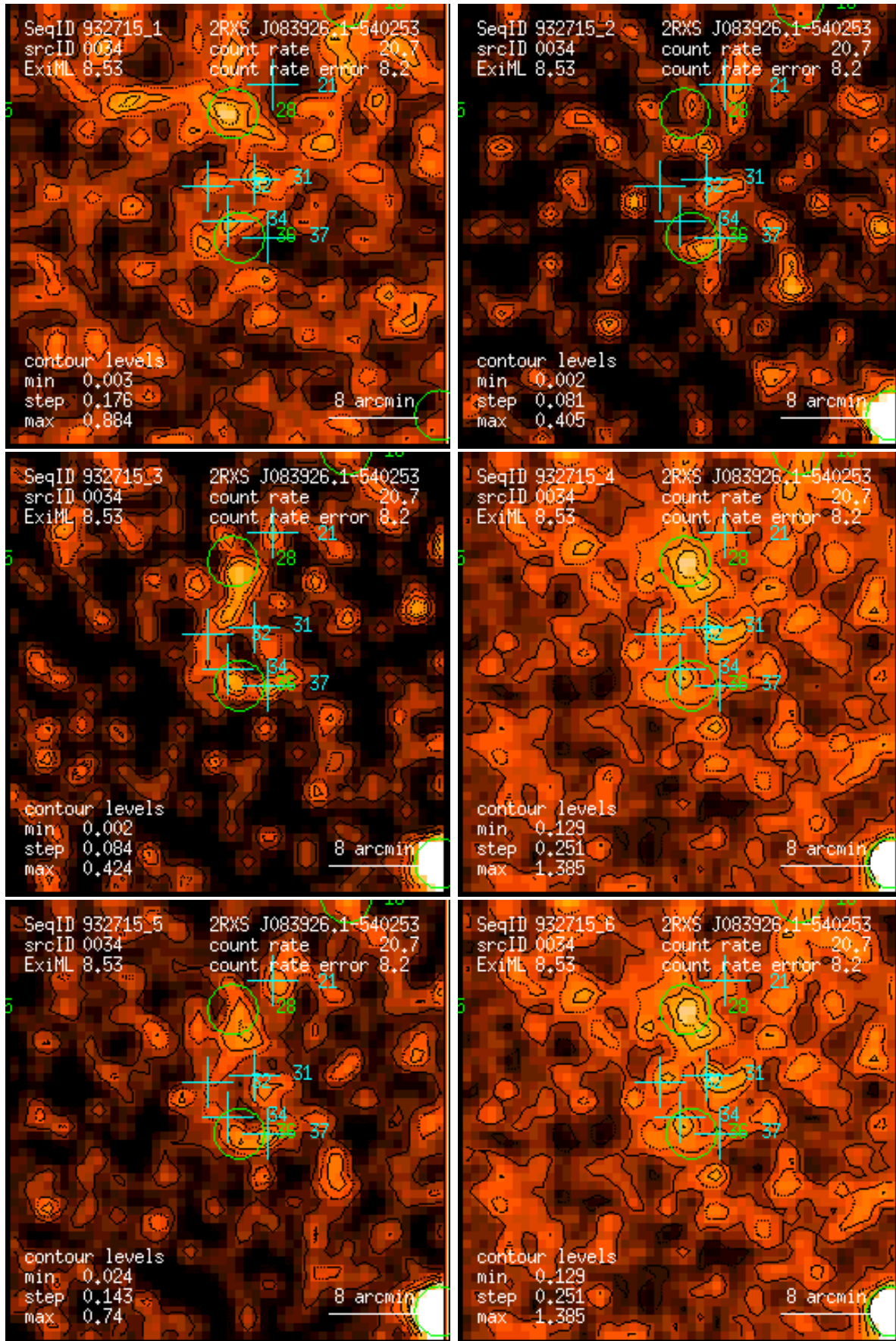
Figure 34: RASS 932715: detection 0034: band rate images, Gaussian filter: (1) PSPC channels 11 – 41, (2) 52 – 90, (3) 91 – 201, (4) 11 – 235, (5) 52 – 201, (6) 11 – 201. Broad band rates in counts/ks. Band rate contour levels in counts/ks/arcmin 2 .
