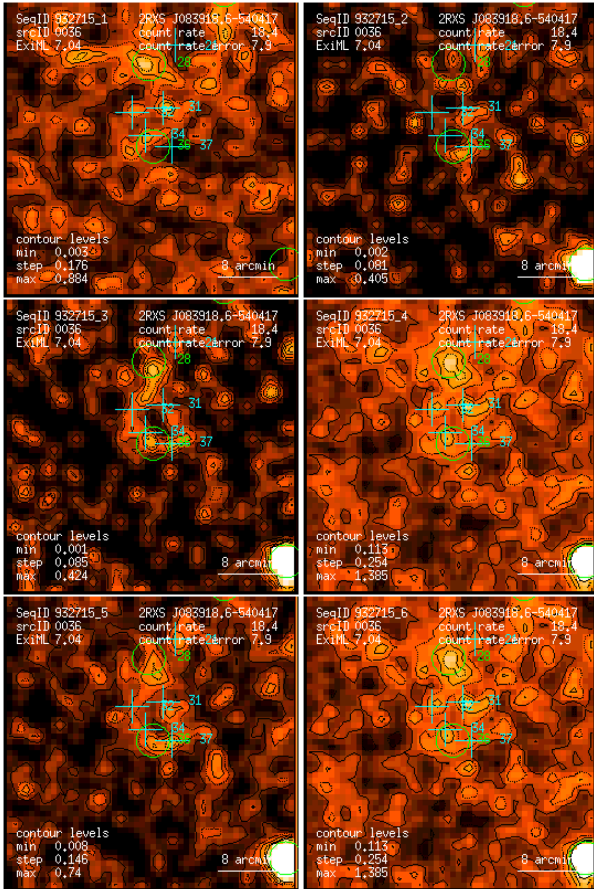
Figure 36: RASS 932715: detection 0036: band rate images, Gaussian filter: (1) PSPC channels 11 – 41, (2) 52 – 90, (3) 91 – 201, (4) 11 – 235, (5) 52 – 201, (6) 11 – 201. Broad band rates in counts/ks. Band rate contour levels in counts/ks/arcmin 2 .
