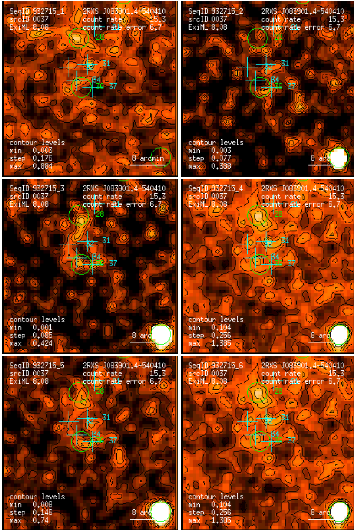
Figure 37: RASS 932715: detection 0037: band rate images, Gaussian filter: (1) PSPC channels 11 – 41, (2) 52 – 90, (3) 91 – 201, (4) 11 – 235, (5) 52 – 201, (6) 11 – 201. Broad band rates in counts/ks. Band rate contour levels in counts/ks/arcmin 2 .
