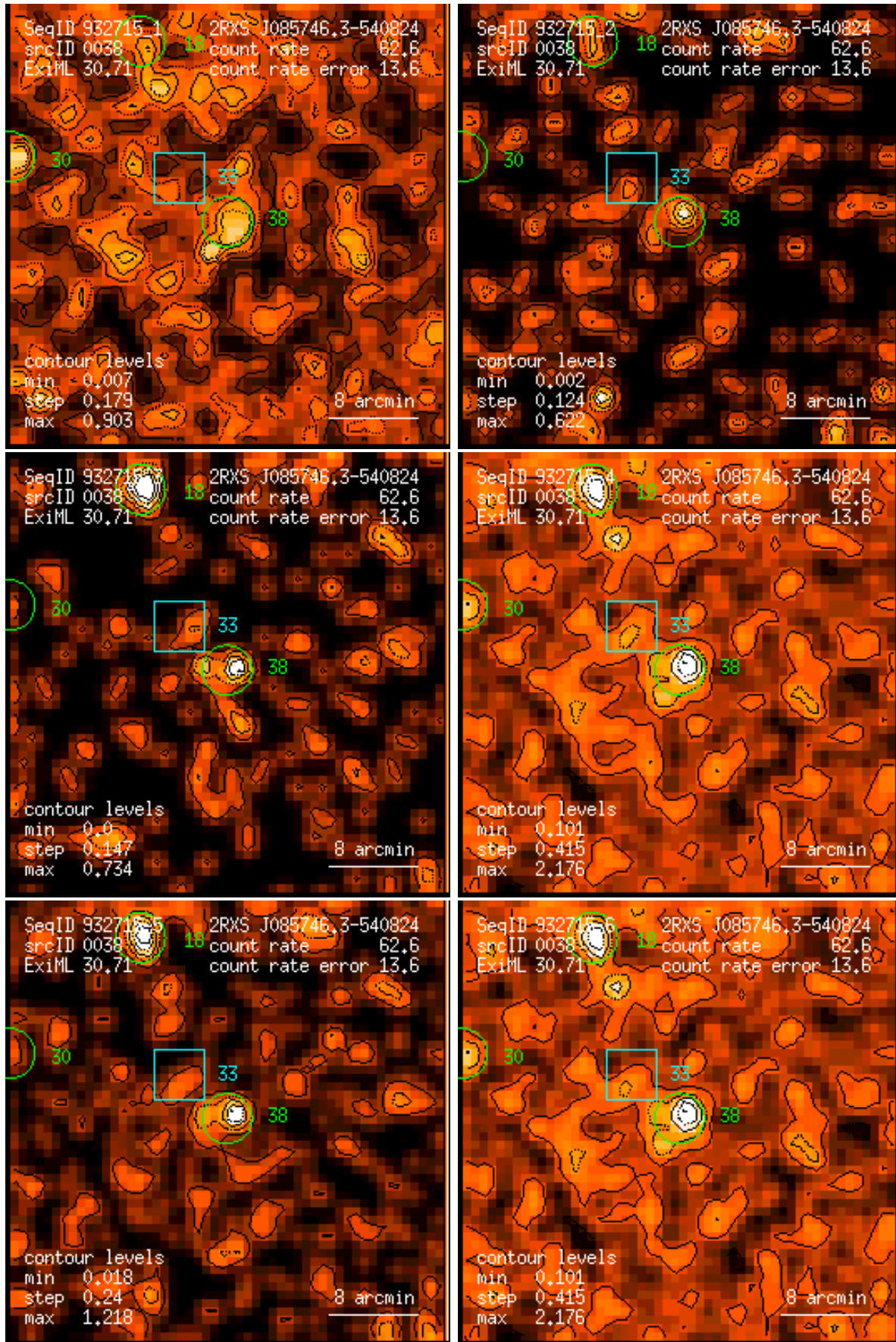
Figure 38: RASS 932715: detection 0038: band rate images, Gaussian filter: (1) PSPC channels 11 – 41, (2) 52 – 90, (3) 91 – 201, (4) 11 – 235, (5) 52 – 201, (6) 11 – 201. Broad band rates in counts/ks. Band rate contour levels in counts/ks/arcmin 2 .
