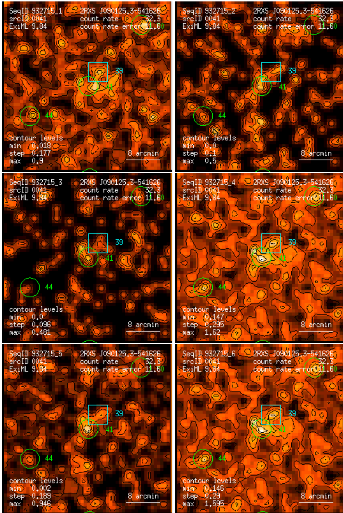
Figure 41: RASS 932715: detection 0041: band rate images, Gaussian filter: (1) PSPC channels 11 – 41, (2) 52 – 90, (3) 91 – 201, (4) 11 – 235, (5) 52 – 201, (6) 11 – 201. Broad band rates in counts/ks. Band rate contour levels in counts/ks/arcmin 2 .
