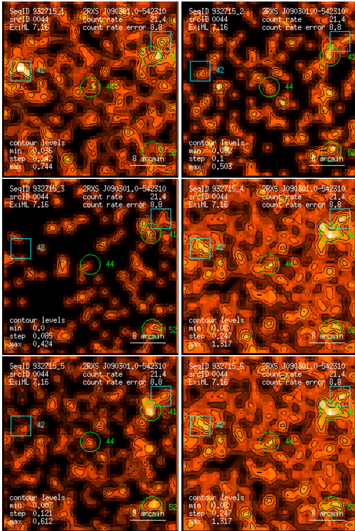
Figure 44: RASS 932715: detection 0044: band rate images, Gaussian filter: (1) PSPC channels 11 – 41, (2) 52 – 90, (3) 91 – 201, (4) 11 – 235, (5) 52 – 201, (6) 11 – 201. Broad band rates in counts/ks. Band rate contour levels in counts/ks/arcmin 2 .
