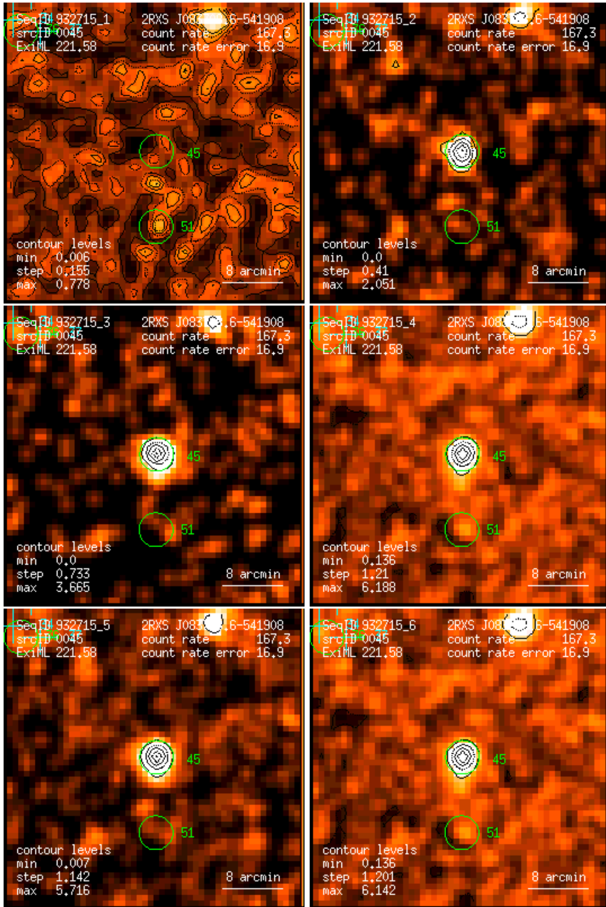
Figure 45: RASS 932715: detection 0045: band rate images, Gaussian filter: (1) PSPC channels 11 – 41, (2) 52 – 90, (3) 91 – 201, (4) 11 – 235, (5) 52 – 201, (6) 11 – 201. Broad band rates in counts/ks. Band rate contour levels in counts/ks/arcmin 2 .
