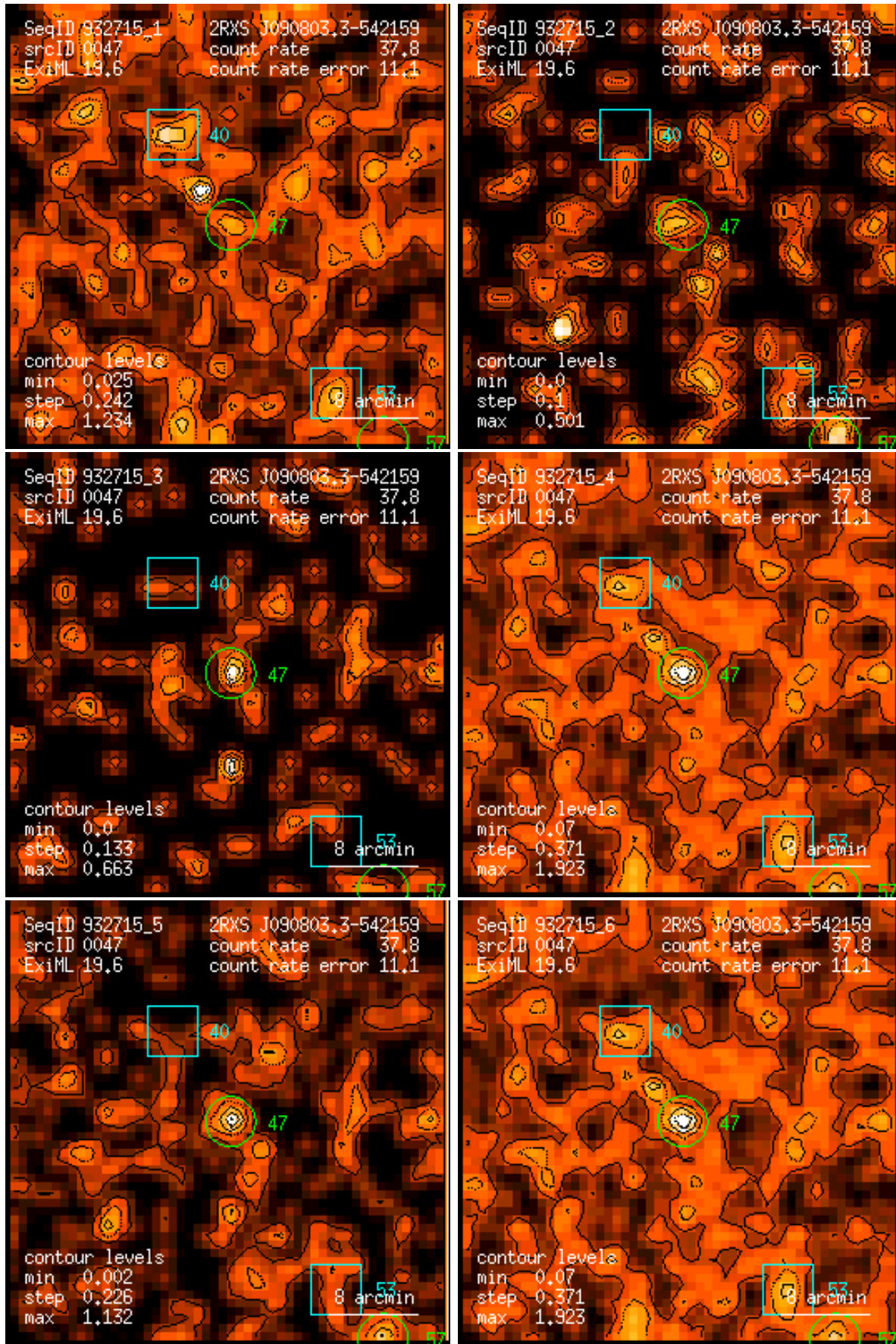
Figure 47: RASS 932715: detection 0047: band rate images, Gaussian filter: (1) PSPC channels 11 – 41, (2) 52 – 90, (3) 91 – 201, (4) 11 – 235, (5) 52 – 201, (6) 11 – 201. Broad band rates in counts/ks. Band rate contour levels in counts/ks/arcmin 2 .
