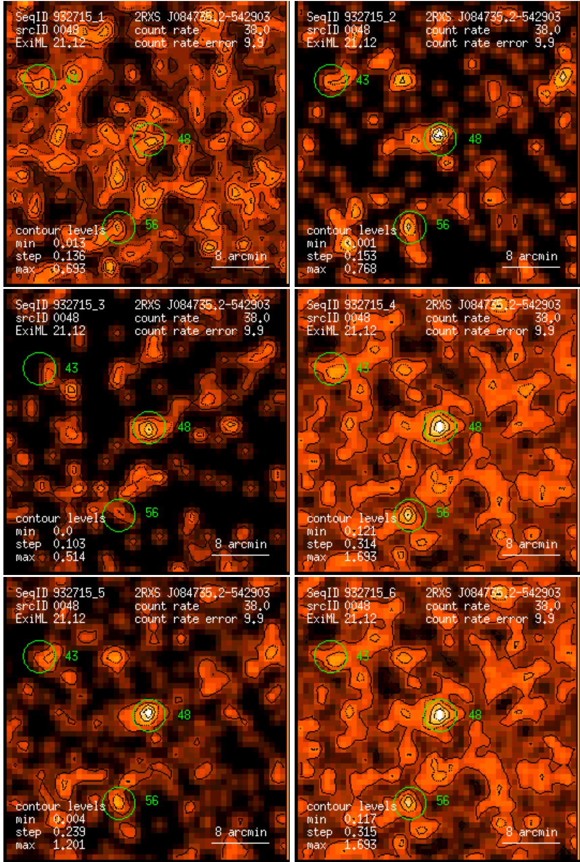
Figure 48: RASS 932715: detection 0048: band rate images, Gaussian filter: (1) PSPC channels 11 – 41, (2) 52 – 90, (3) 91 – 201, (4) 11 – 235, (5) 52 – 201, (6) 11 – 201. Broad band rates in counts/ks. Band rate contour levels in counts/ks/arcmin 2 .
