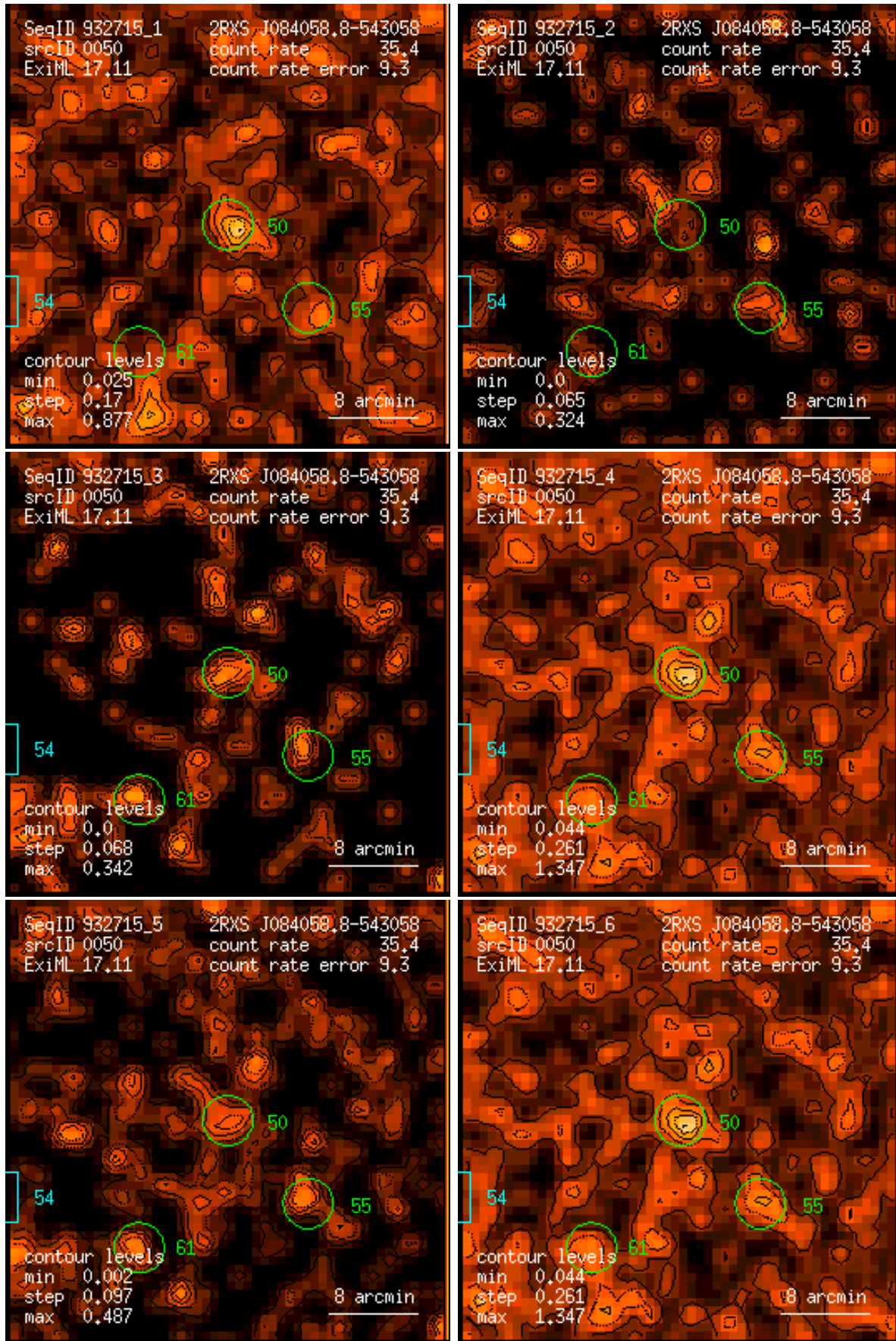
Figure 50: RASS 932715: detection 0050: band rate images, Gaussian filter: (1) PSPC channels 11 – 41, (2) 52 – 90, (3) 91 – 201, (4) 11 – 235, (5) 52 – 201, (6) 11 – 201. Broad band rates in counts/ks. Band rate contour levels in counts/ks/arcmin 2 .
