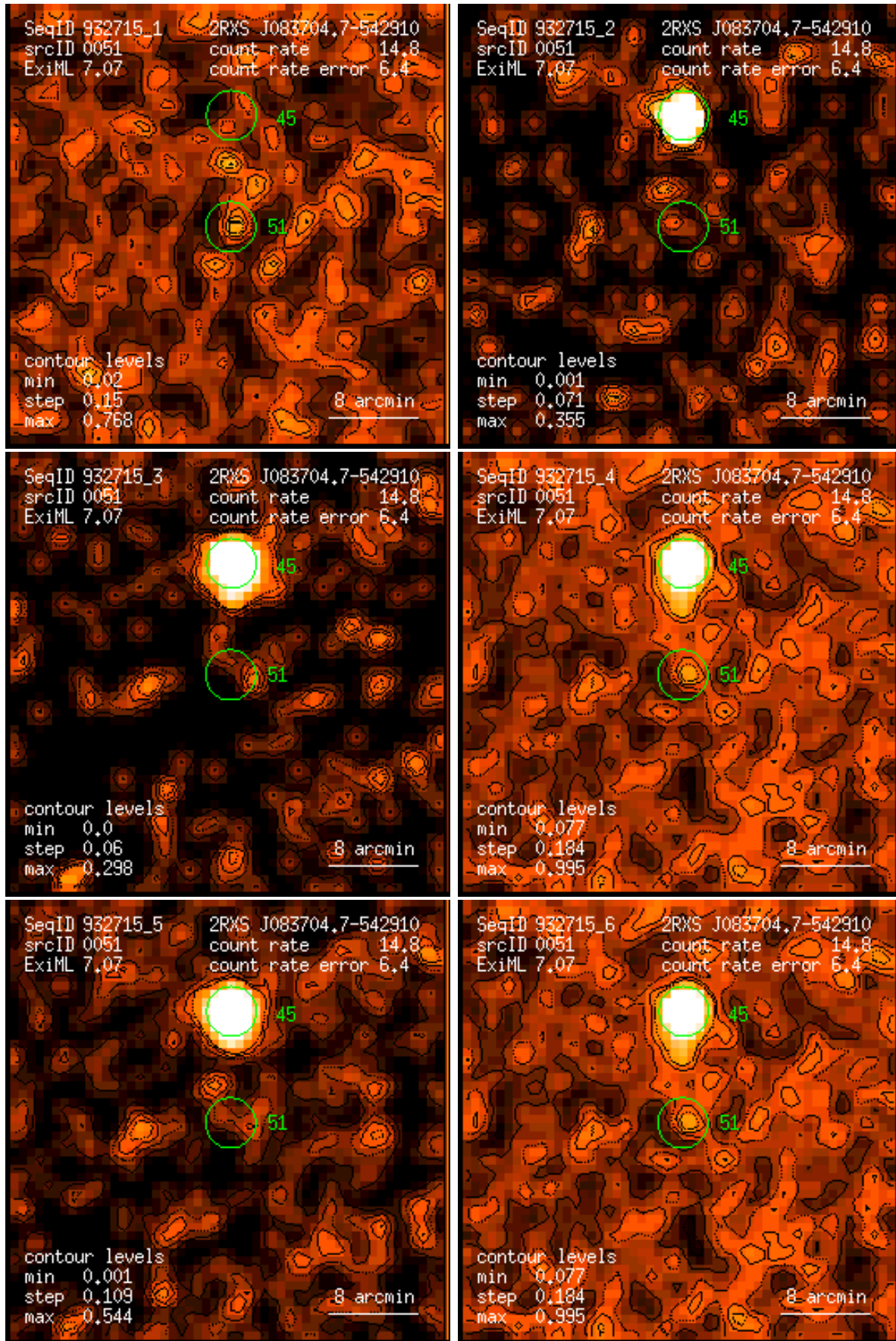
Figure 51: RASS 932715: detection 0051: band rate images, Gaussian filter: (1) PSPC channels 11 – 41, (2) 52 – 90, (3) 91 – 201, (4) 11 – 235, (5) 52 – 201, (6) 11 – 201. Broad band rates in counts/ks. Band rate contour levels in counts/ks/arcmin 2 .
