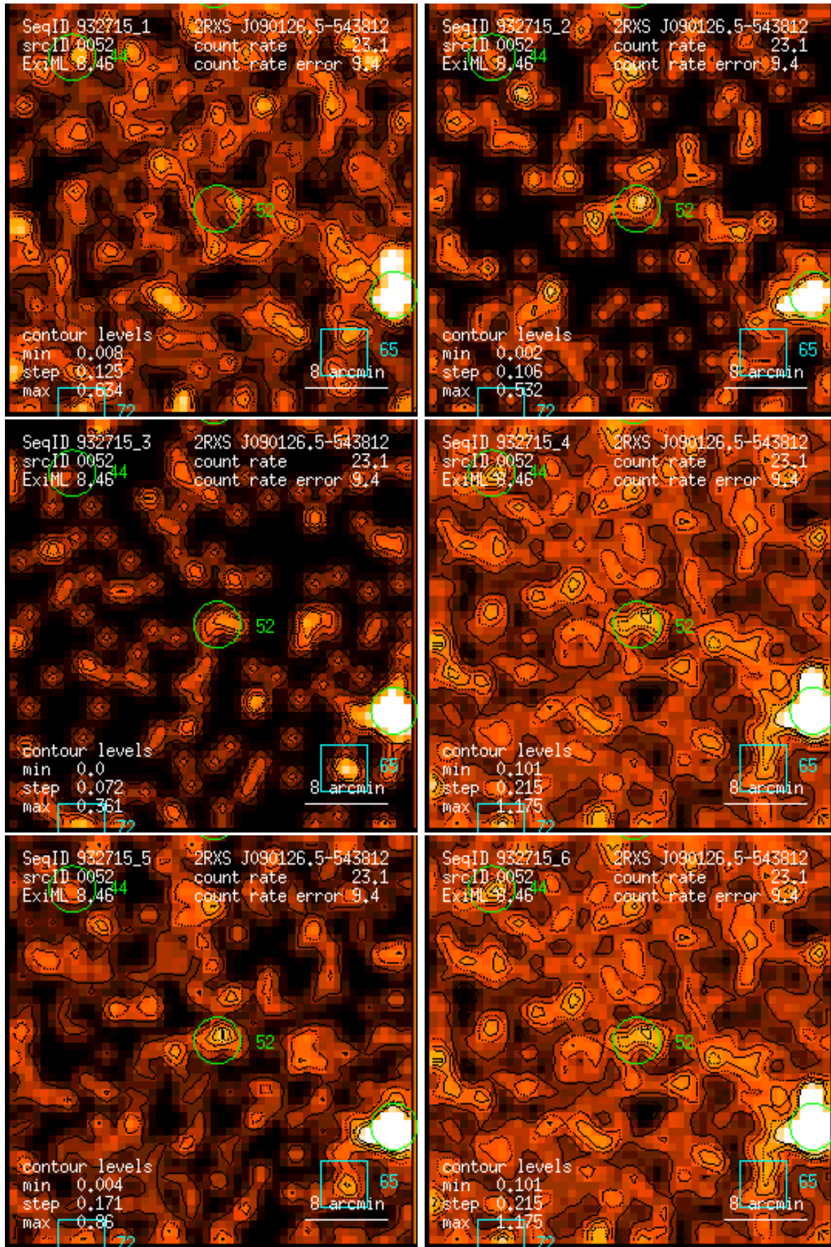
Figure 52: RASS 932715: detection 0052: band rate images, Gaussian filter: (1) PSPC channels 11 – 41, (2) 52 – 90, (3) 91 – 201, (4) 11 – 235, (5) 52 – 201, (6) 11 – 201. Broad band rates in counts/ks. Band rate contour levels in counts/ks/arcmin 2 .
