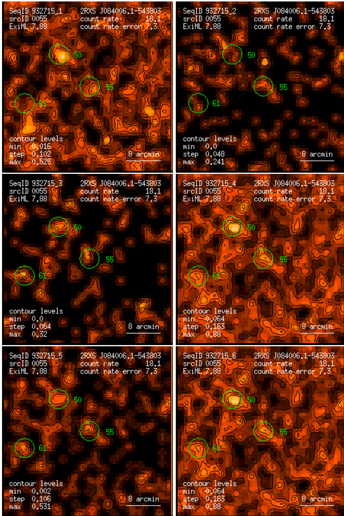
Figure 55: RASS 932715: detection 0055: band rate images, Gaussian filter: (1) PSPC channels 11 – 41, (2) 52 – 90, (3) 91 – 201, (4) 11 – 235, (5) 52 – 201, (6) 11 – 201. Broad band rates in counts/ks. Band rate contour levels in counts/ks/arcmin 2 .
