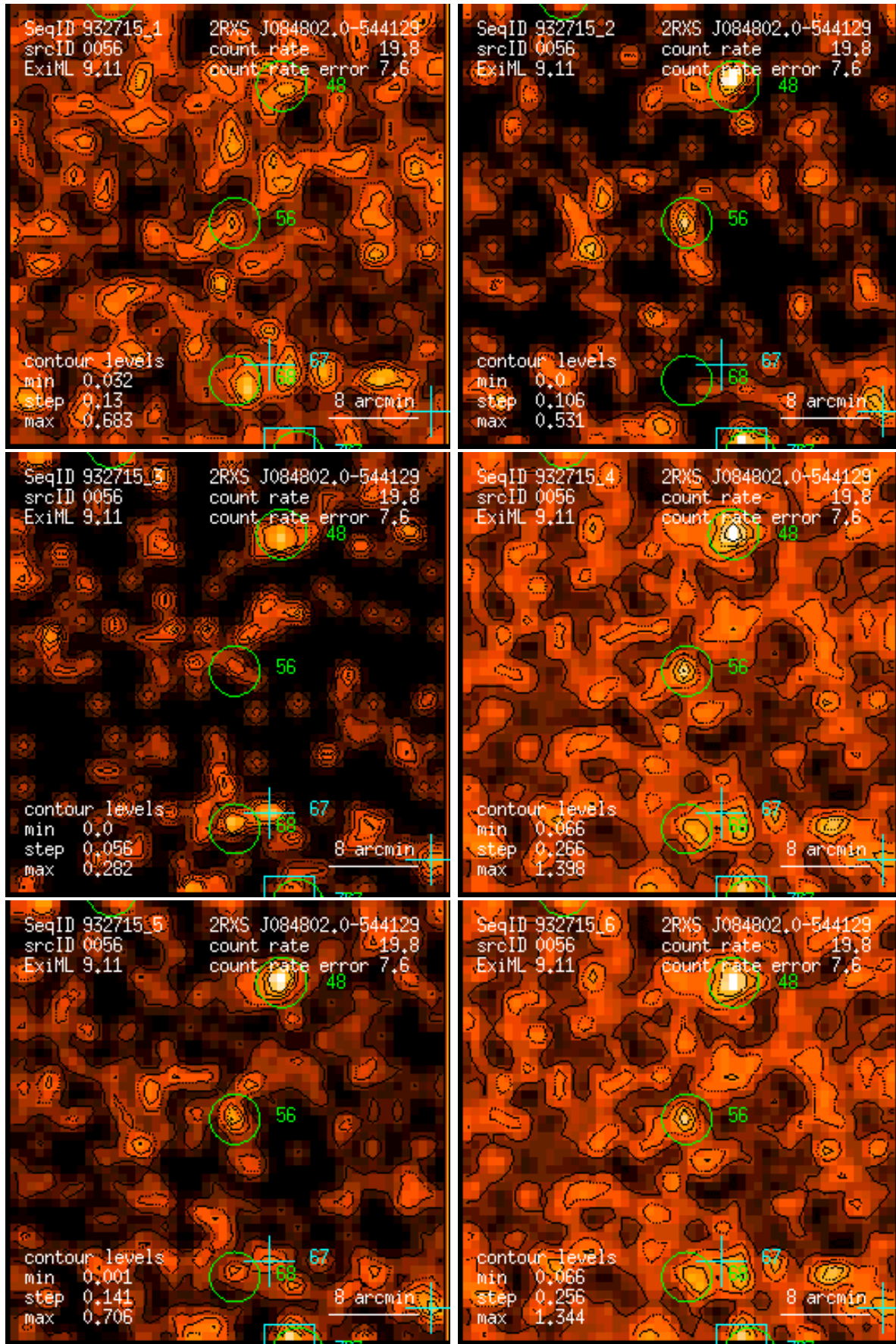
Figure 56: RASS 932715: detection 0056: band rate images, Gaussian filter: (1) PSPC channels 11 – 41, (2) 52 – 90, (3) 91 – 201, (4) 11 – 235, (5) 52 – 201, (6) 11 – 201. Broad band rates in counts/ks. Band rate contour levels in counts/ks/arcmin 2 .
