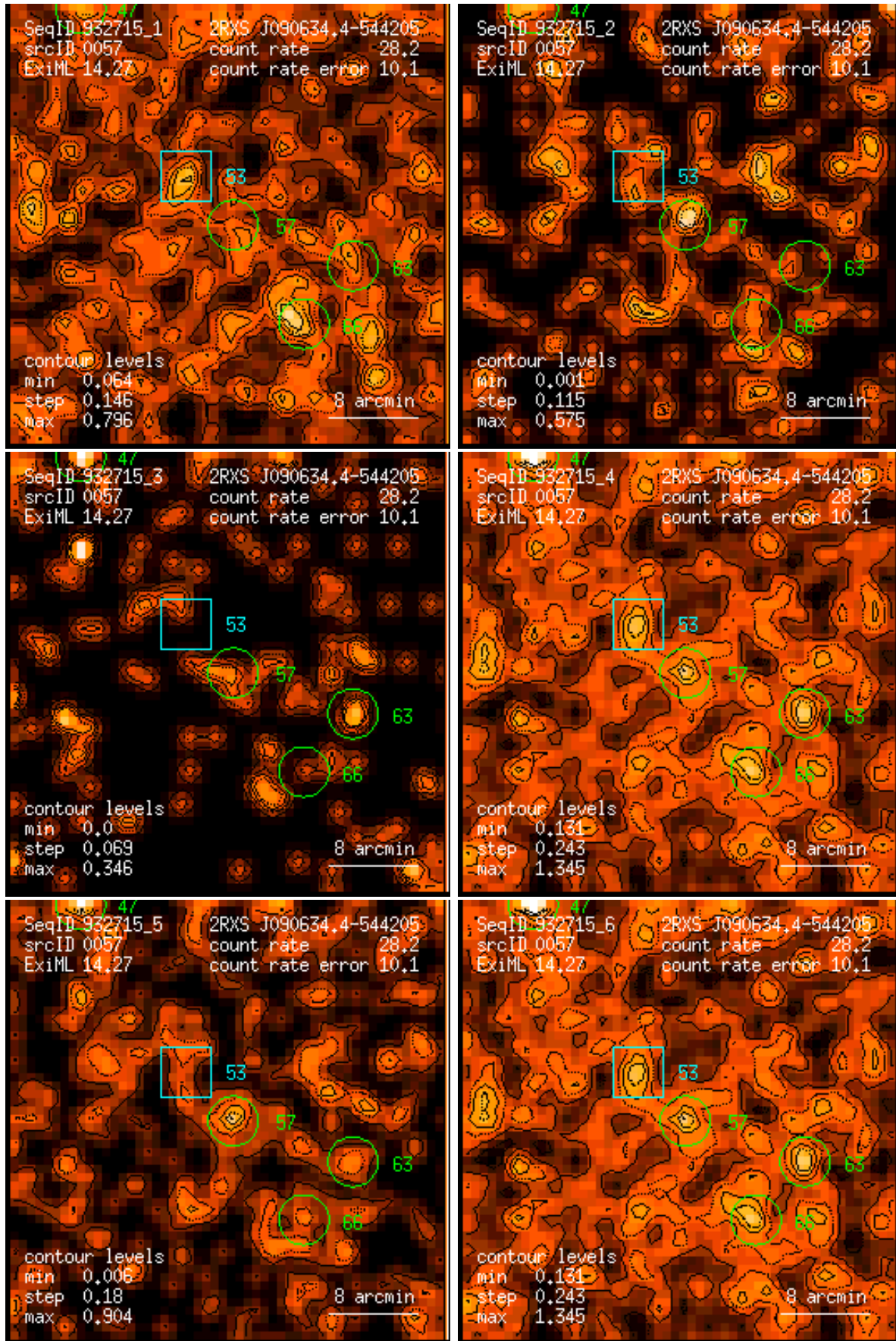
Figure 57: RASS 932715: detection 0057: band rate images, Gaussian filter: (1) PSPC channels 11 – 41, (2) 52 – 90, (3) 91 – 201, (4) 11 – 235, (5) 52 – 201, (6) 11 – 201. Broad band rates in counts/ks. Band rate contour levels in counts/ks/arcmin 2 .
