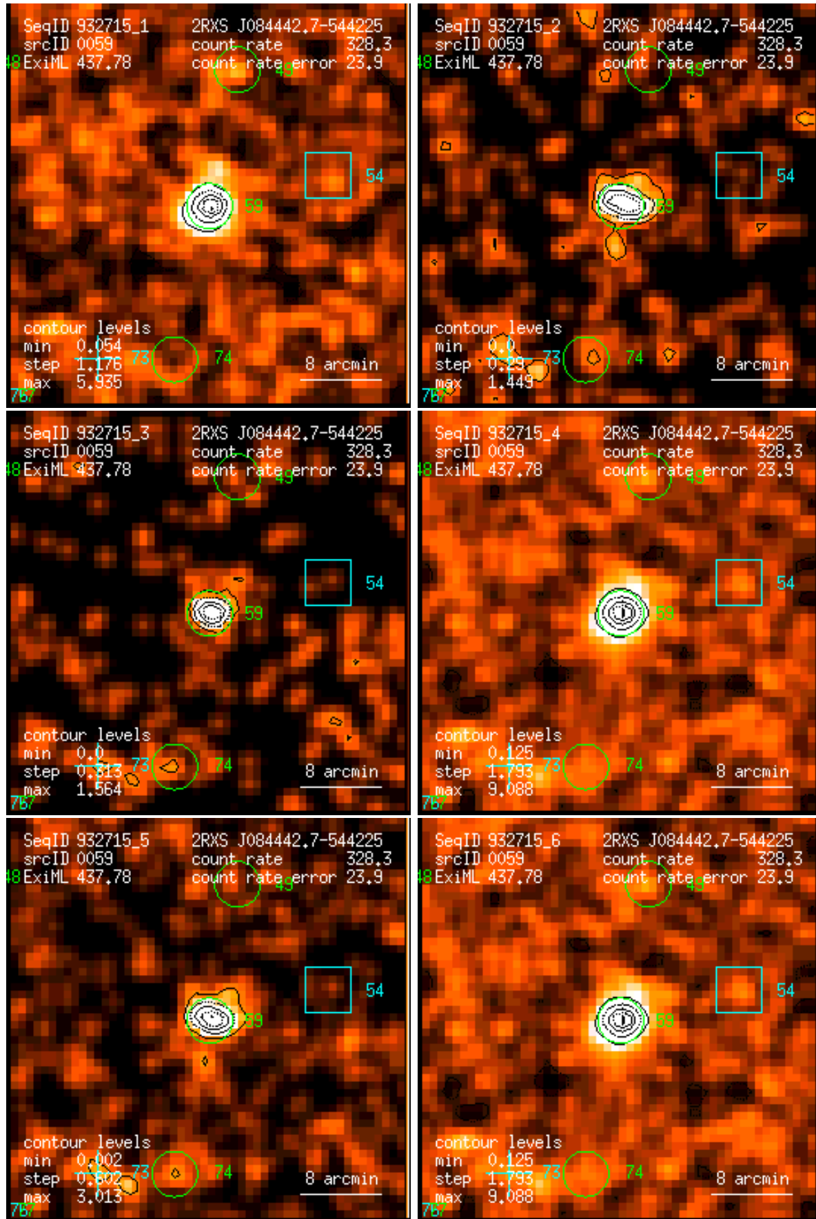
Figure 59: RASS 932715: detection 0059: band rate images, Gaussian filter: (1) PSPC channels 11 – 41, (2) 52 – 90, (3) 91 – 201, (4) 11 – 235, (5) 52 – 201, (6) 11 – 201. Broad band rates in counts/ks. Band rate contour levels in counts/ks/arcmin 2 .
