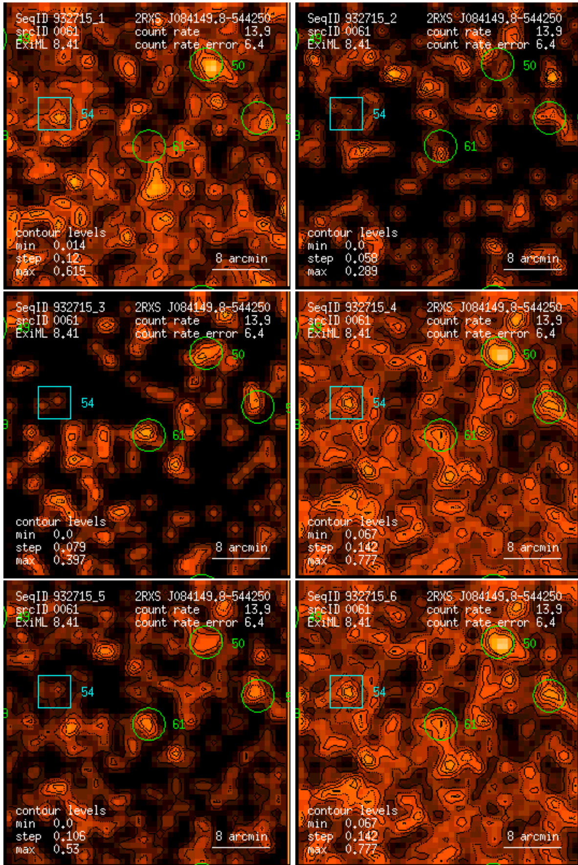
Figure 61: RASS 932715: detection 0061: band rate images, Gaussian filter: (1) PSPC channels 11 – 41, (2) 52 – 90, (3) 91 – 201, (4) 11 – 235, (5) 52 – 201, (6) 11 – 201. Broad band rates in counts/ks. Band rate contour levels in counts/ks/arcmin 2 .
