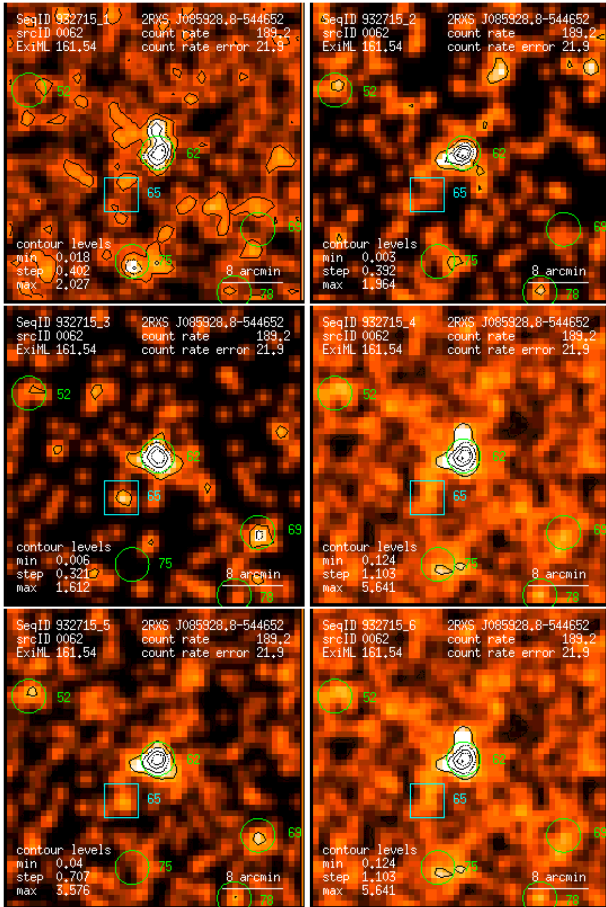
Figure 62: RASS 932715: detection 0062: band rate images, Gaussian filter: (1) PSPC channels 11 – 41, (2) 52 – 90, (3) 91 – 201, (4) 11 – 235, (5) 52 – 201, (6) 11 – 201. Broad band rates in counts/ks. Band rate contour levels in counts/ks/arcmin 2 .
