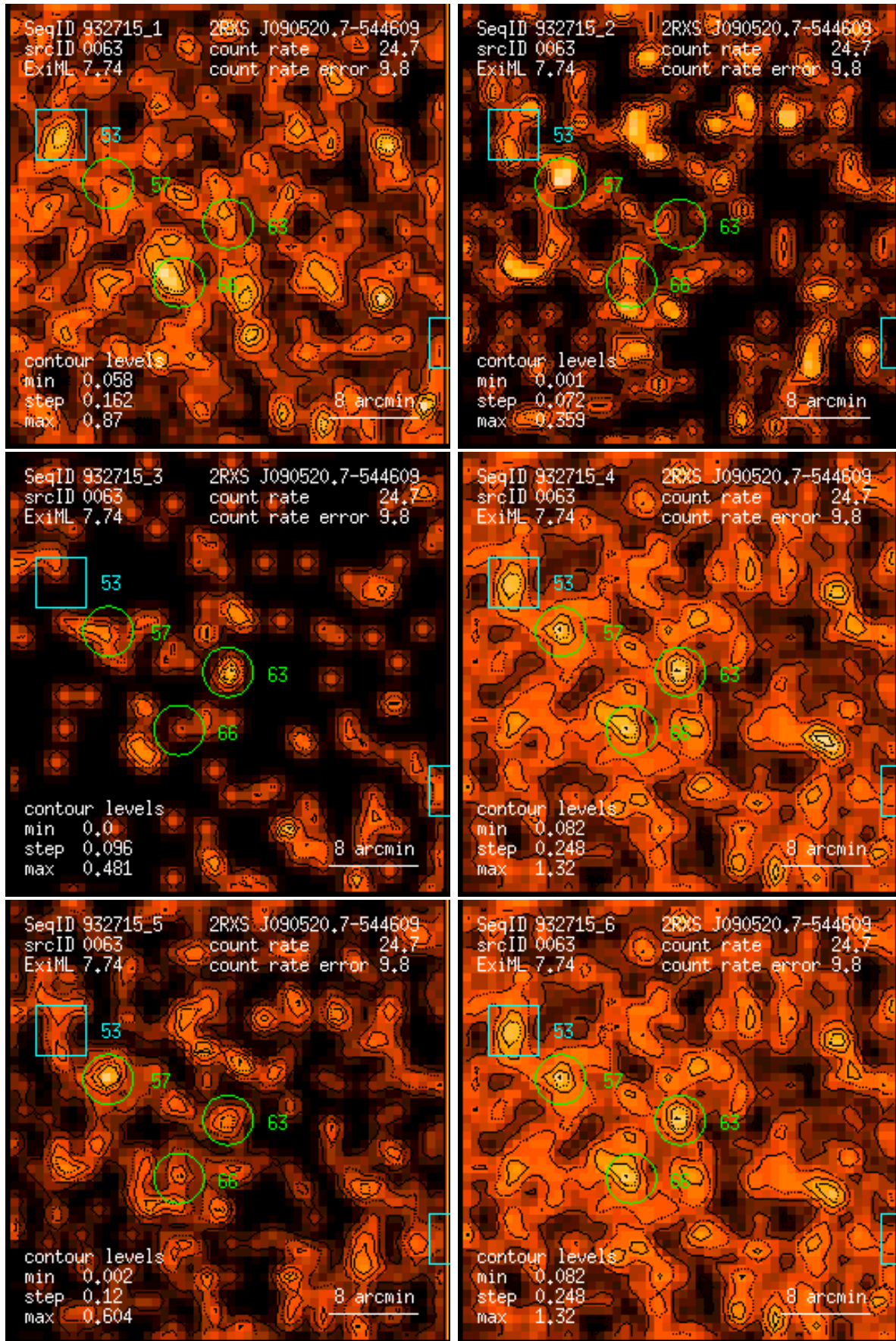
Figure 63: RASS 932715: detection 0063: band rate images, Gaussian filter: (1) PSPC channels 11 – 41, (2) 52 – 90, (3) 91 – 201, (4) 11 – 235, (5) 52 – 201, (6) 11 – 201. Broad band rates in counts/ks. Band rate contour levels in counts/ks/arcmin 2 .
