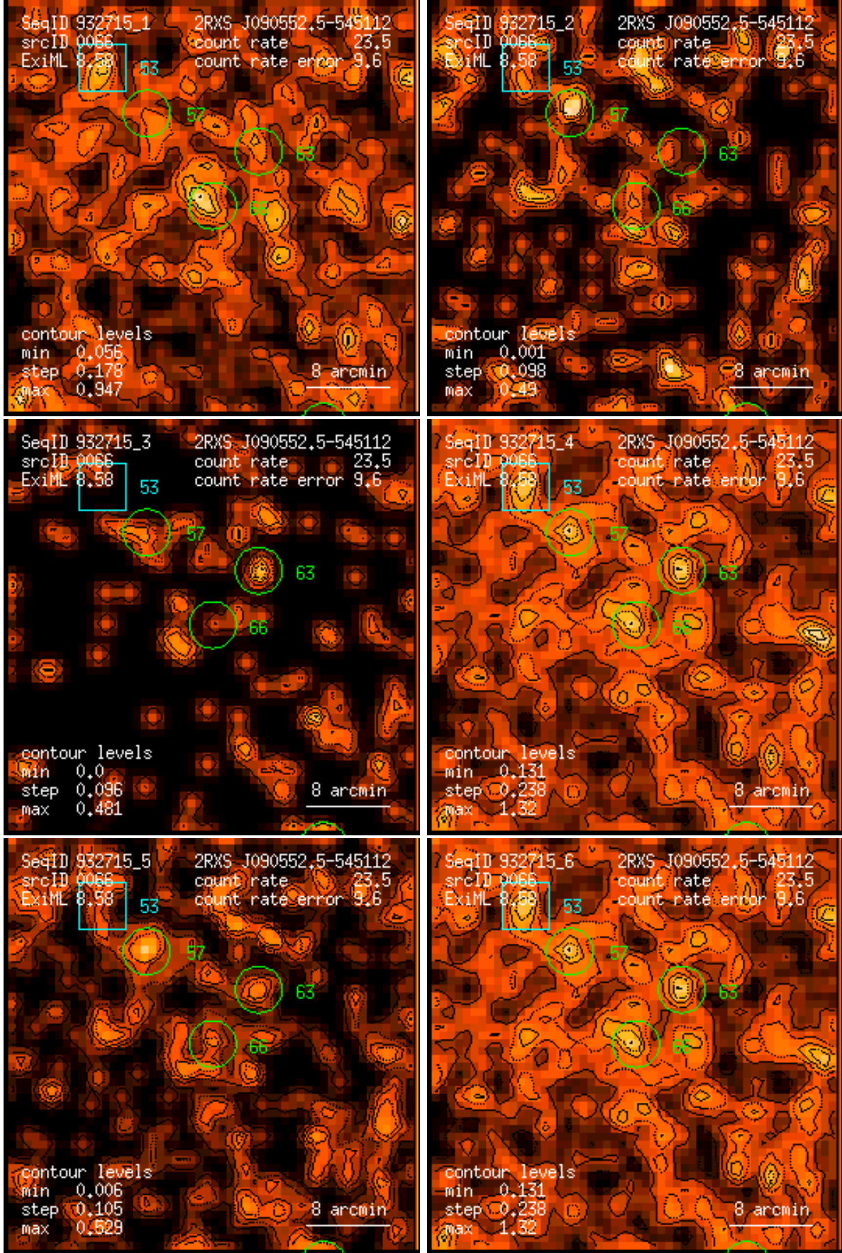
Figure 66: RASS 932715: detection 0066: band rate images, Gaussian filter: (1) PSPC channels 11 – 41, (2) 52 – 90, (3) 91 – 201, (4) 11 – 235, (5) 52 – 201, (6) 11 – 201. Broad band rates in counts/ks. Band rate contour levels in counts/ks/arcmin 2 .
