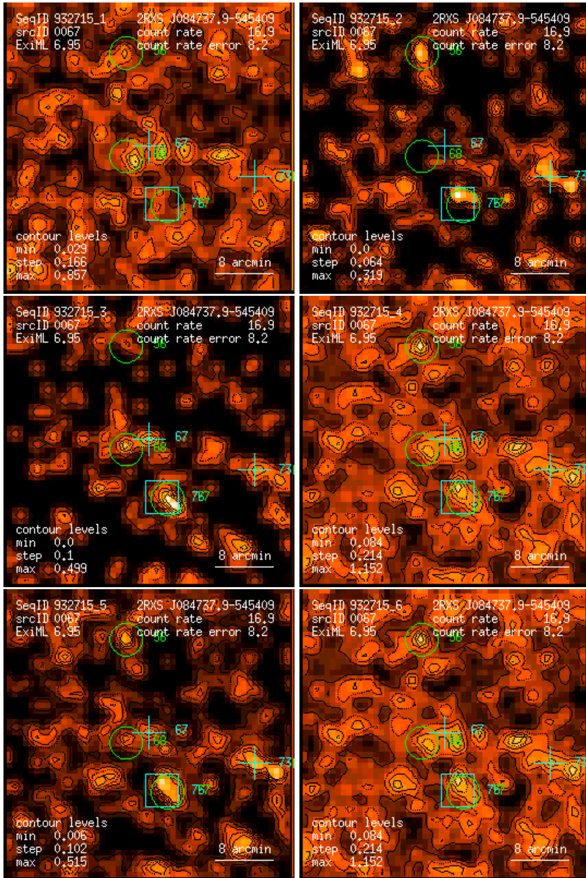
Figure 67: RASS 932715: detection 0067: band rate images, Gaussian filter: (1) PSPC channels 11 – 41, (2) 52 – 90, (3) 91 – 201, (4) 11 – 235, (5) 52 – 201, (6) 11 – 201. Broad band rates in counts/ks. Band rate contour levels in counts/ks/arcmin 2 .
