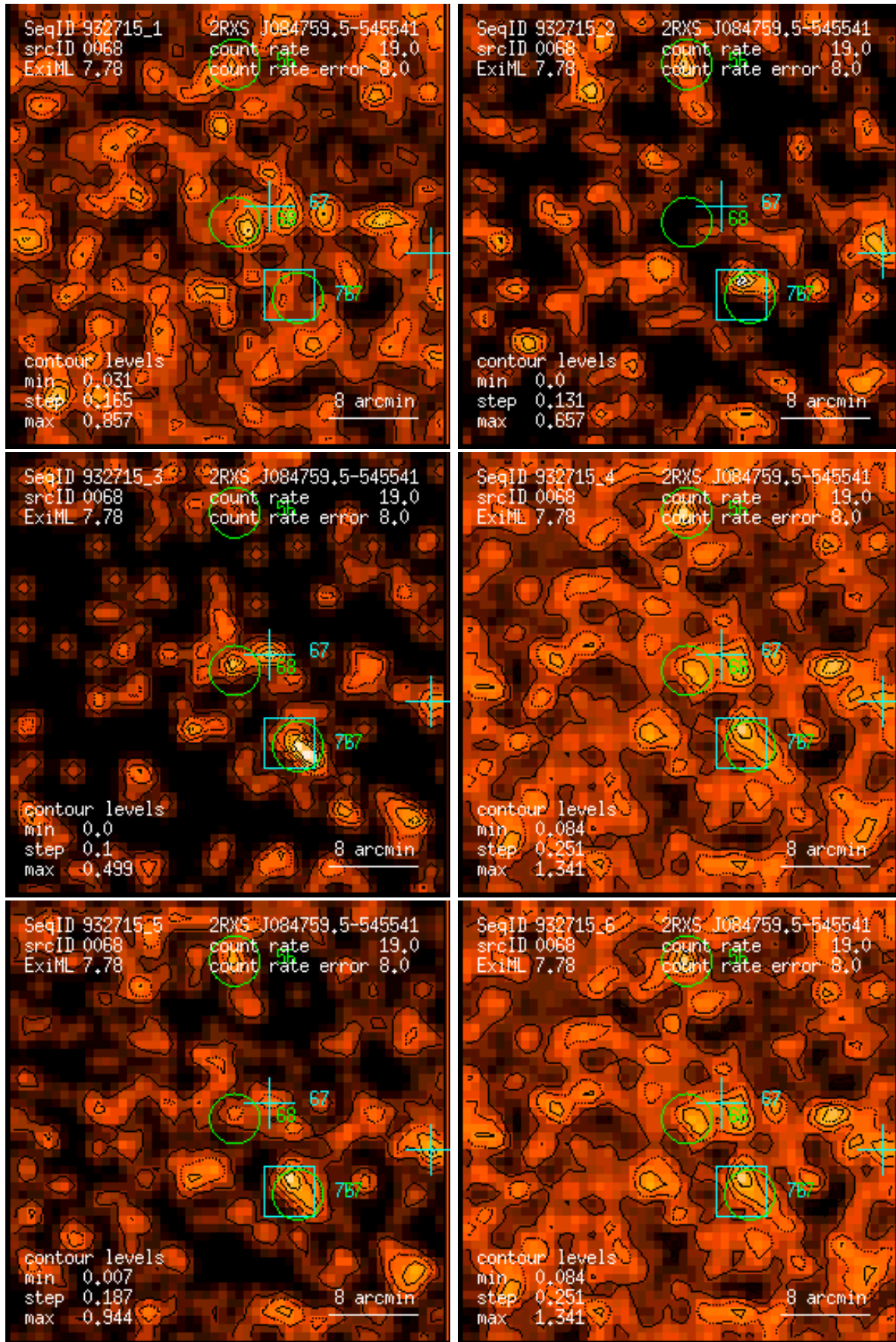
Figure 68: RASS 932715: detection 0068: band rate images, Gaussian filter: (1) PSPC channels 11 – 41, (2) 52 – 90, (3) 91 – 201, (4) 11 – 235, (5) 52 – 201, (6) 11 – 201. Broad band rates in counts/ks. Band rate contour levels in counts/ks/arcmin 2 .
