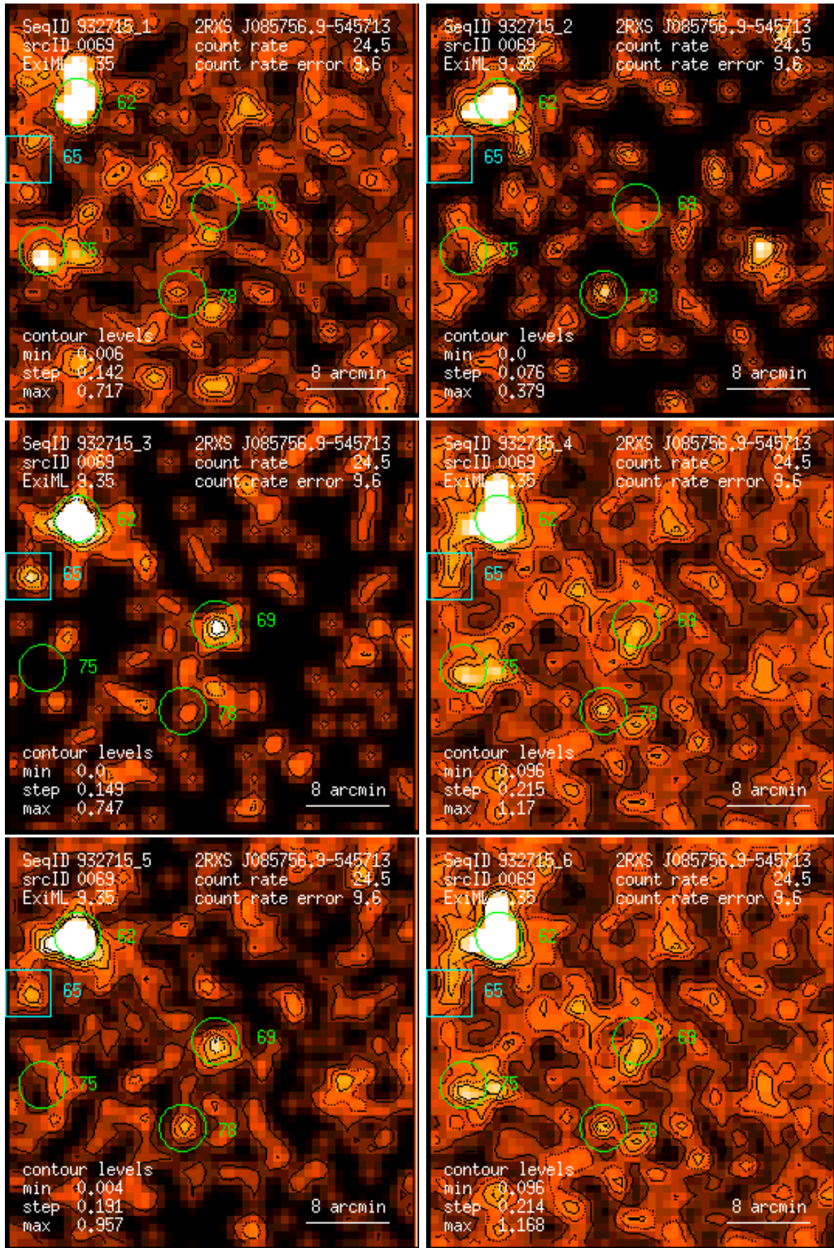
Figure 69: RASS 932715: detection 0069: band rate images, Gaussian filter: (1) PSPC channels 11 – 41, (2) 52 – 90, (3) 91 – 201, (4) 11 – 235, (5) 52 – 201, (6) 11 – 201. Broad band rates in counts/ks. Band rate contour levels in counts/ks/arcmin 2 .
