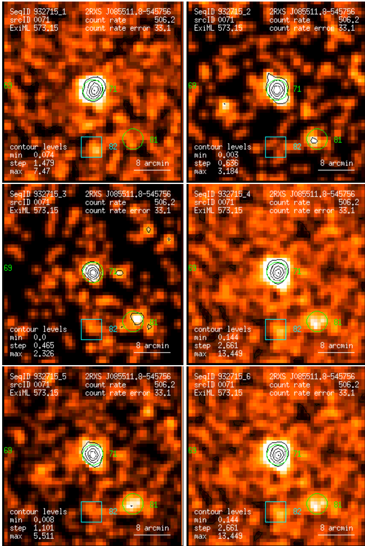
Figure 71: RASS 932715: detection 0071: band rate images, Gaussian filter: (1) PSPC channels 11 – 41, (2) 52 – 90, (3) 91 – 201, (4) 11 – 235, (5) 52 – 201, (6) 11 – 201. Broad band rates in counts/ks. Band rate contour levels in counts/ks/arcmin 2 .
