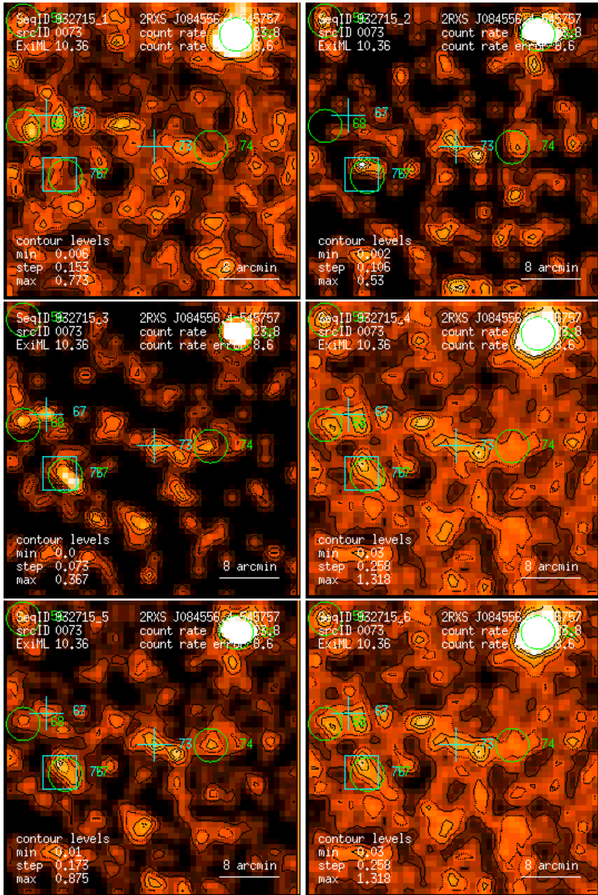
Figure 73: RASS 932715: detection 0073: band rate images, Gaussian filter: (1) PSPC channels 11 – 41, (2) 52 – 90, (3) 91 – 201, (4) 11 – 235, (5) 52 – 201, (6) 11 – 201. Broad band rates in counts/ks. Band rate contour levels in counts/ks/arcmin 2 .
