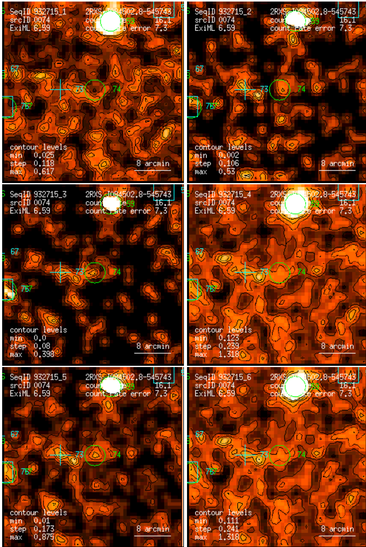
Figure 74: RASS 932715: detection 0074: band rate images, Gaussian filter: (1) PSPC channels 11 – 41, (2) 52 – 90, (3) 91 – 201, (4) 11 – 235, (5) 52 – 201, (6) 11 – 201. Broad band rates in counts/ks. Band rate contour levels in counts/ks/arcmin 2 .
