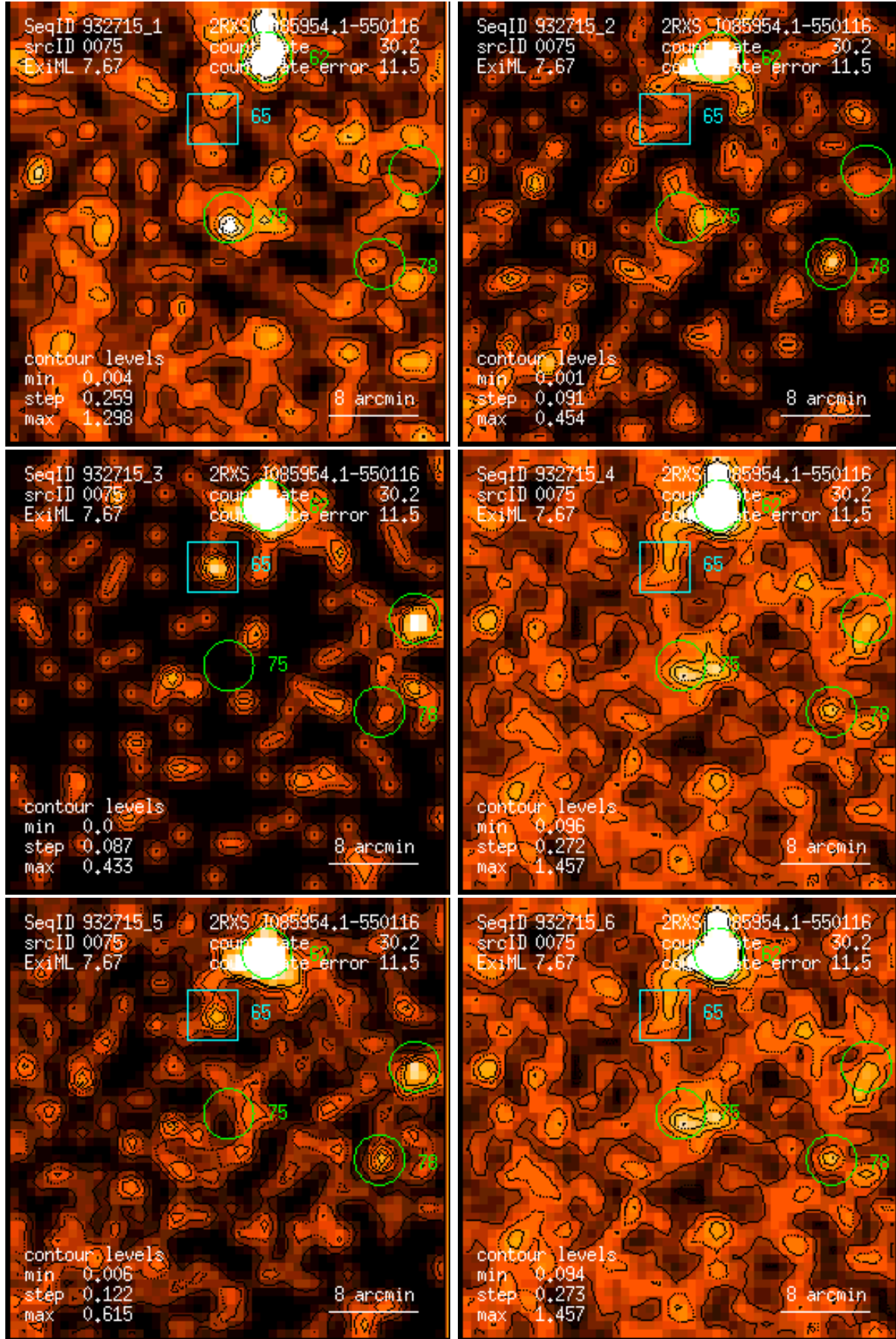
Figure 75: RASS 932715: detection 0075: band rate images, Gaussian filter: (1) PSPC channels 11 – 41, (2) 52 – 90, (3) 91 – 201, (4) 11 – 235, (5) 52 – 201, (6) 11 – 201. Broad band rates in counts/ks. Band rate contour levels in counts/ks/arcmin 2 .
