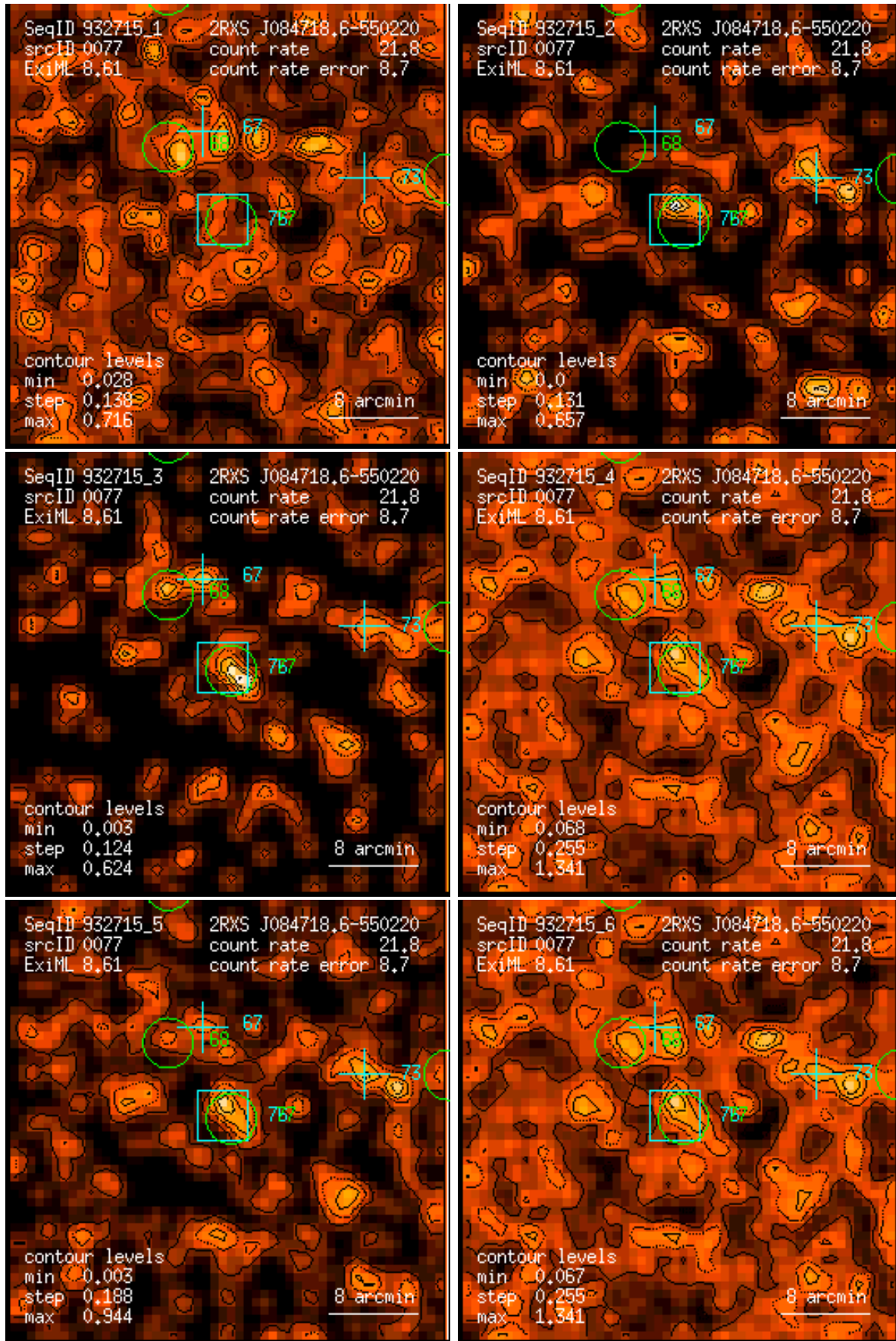
Figure 77: RASS 932715: detection 0077: band rate images, Gaussian filter: (1) PSPC channels 11 – 41, (2) 52 – 90, (3) 91 – 201, (4) 11 – 235, (5) 52 – 201, (6) 11 – 201. Broad band rates in counts/ks. Band rate contour levels in counts/ks/arcmin 2 .
