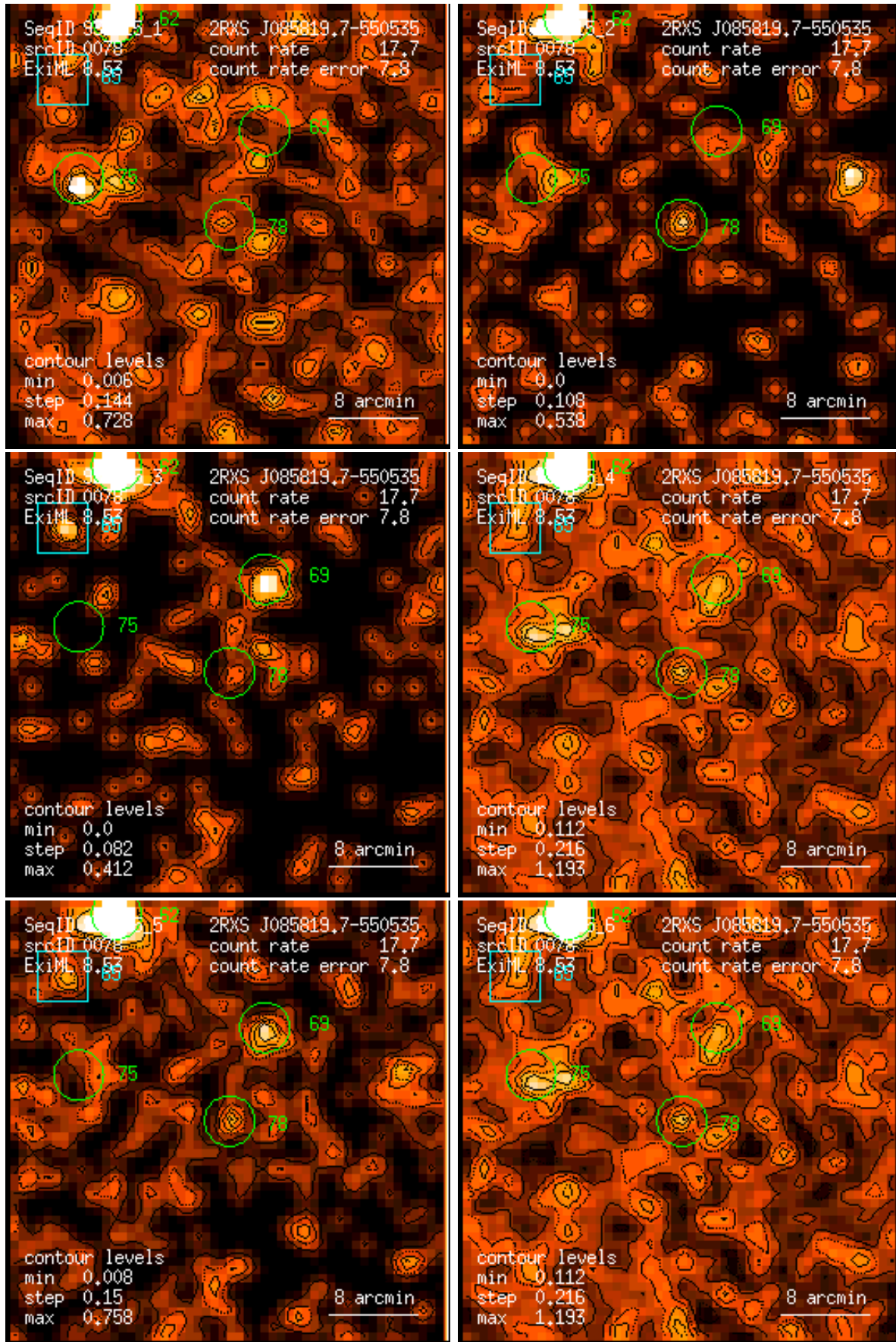
Figure 78: RASS 932715: detection 0078: band rate images, Gaussian filter: (1) PSPC channels 11 – 41, (2) 52 – 90, (3) 91 – 201, (4) 11 – 235, (5) 52 – 201, (6) 11 – 201. Broad band rates in counts/ks. Band rate contour levels in counts/ks/arcmin 2 .
