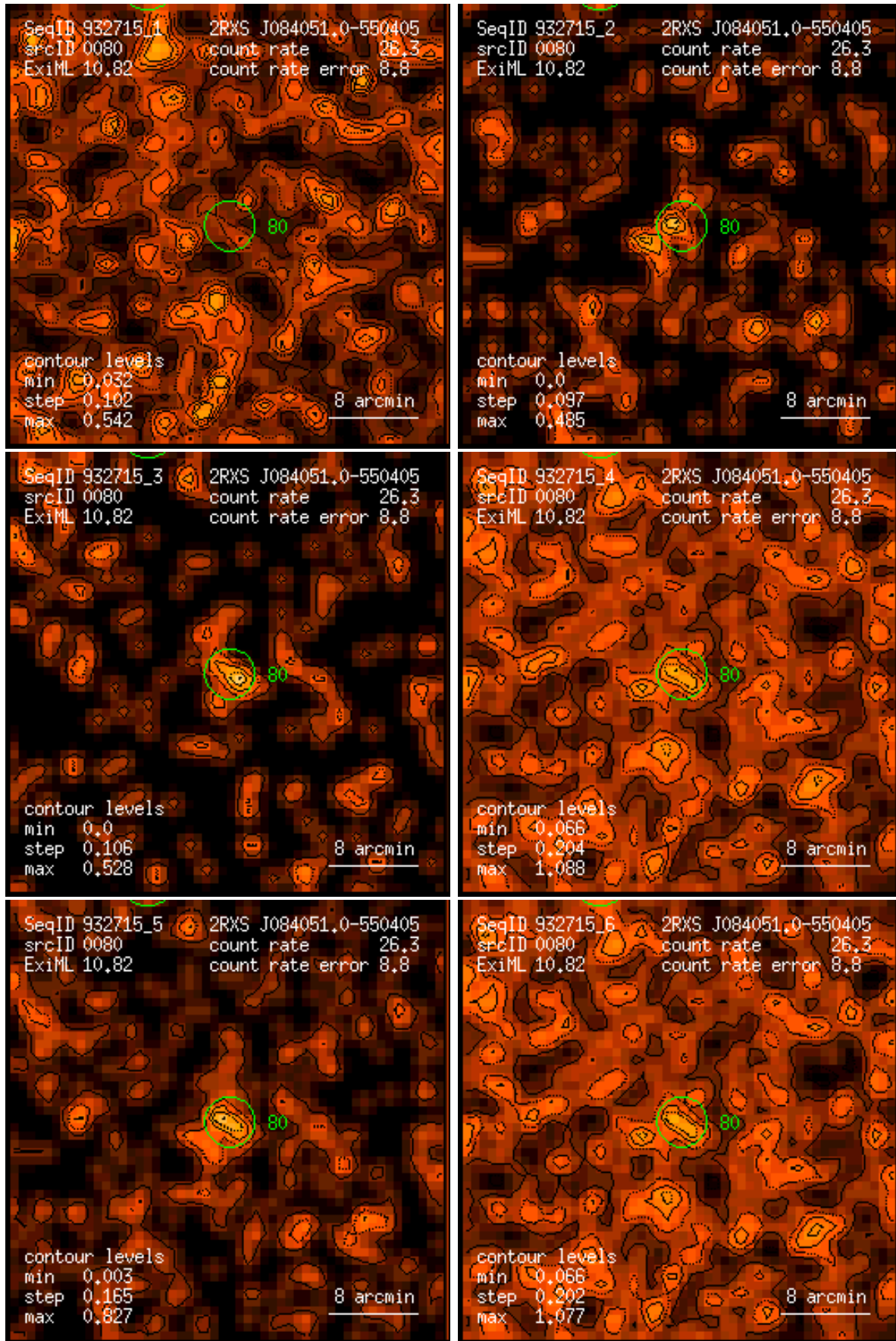
Figure 80: RASS 932715: detection 0080: band rate images, Gaussian filter: (1) PSPC channels 11 – 41, (2) 52 – 90, (3) 91 – 201, (4) 11 – 235, (5) 52 – 201, (6) 11 – 201. Broad band rates in counts/ks. Band rate contour levels in counts/ks/arcmin 2 .
