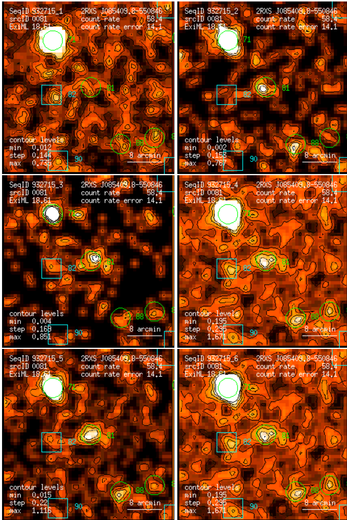
Figure 81: RASS 932715: detection 0081: band rate images, Gaussian filter: (1) PSPC channels 11 – 41, (2) 52 – 90, (3) 91 – 201, (4) 11 – 235, (5) 52 – 201, (6) 11 – 201. Broad band rates in counts/ks. Band rate contour levels in counts/ks/arcmin 2 .
