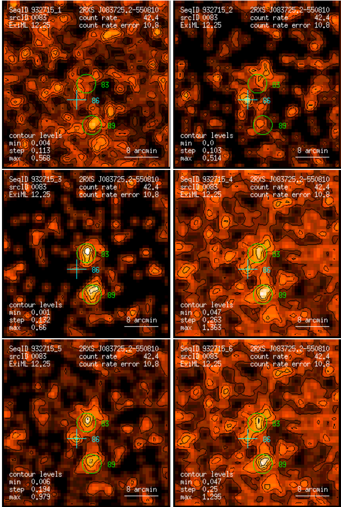
Figure 83: RASS 932715: detection 0083: band rate images, Gaussian filter: (1) PSPC channels 11 – 41, (2) 52 – 90, (3) 91 – 201, (4) 11 – 235, (5) 52 – 201, (6) 11 – 201. Broad band rates in counts/ks. Band rate contour levels in counts/ks/arcmin 2 .
