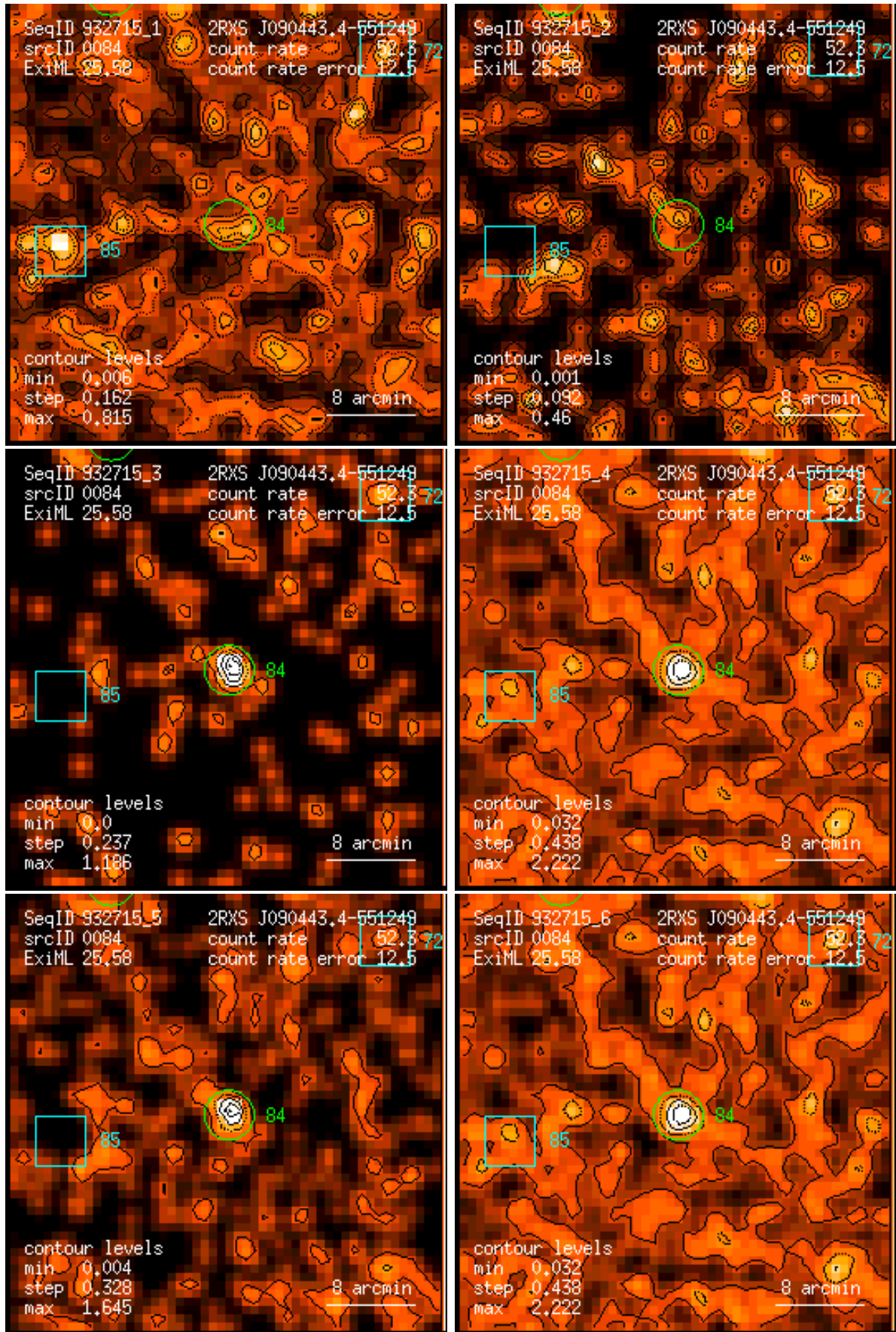
Figure 84: RASS 932715: detection 0084: band rate images, Gaussian filter: (1) PSPC channels 11 – 41, (2) 52 – 90, (3) 91 – 201, (4) 11 – 235, (5) 52 – 201, (6) 11 – 201. Broad band rates in counts/ks. Band rate contour levels in counts/ks/arcmin 2 .
