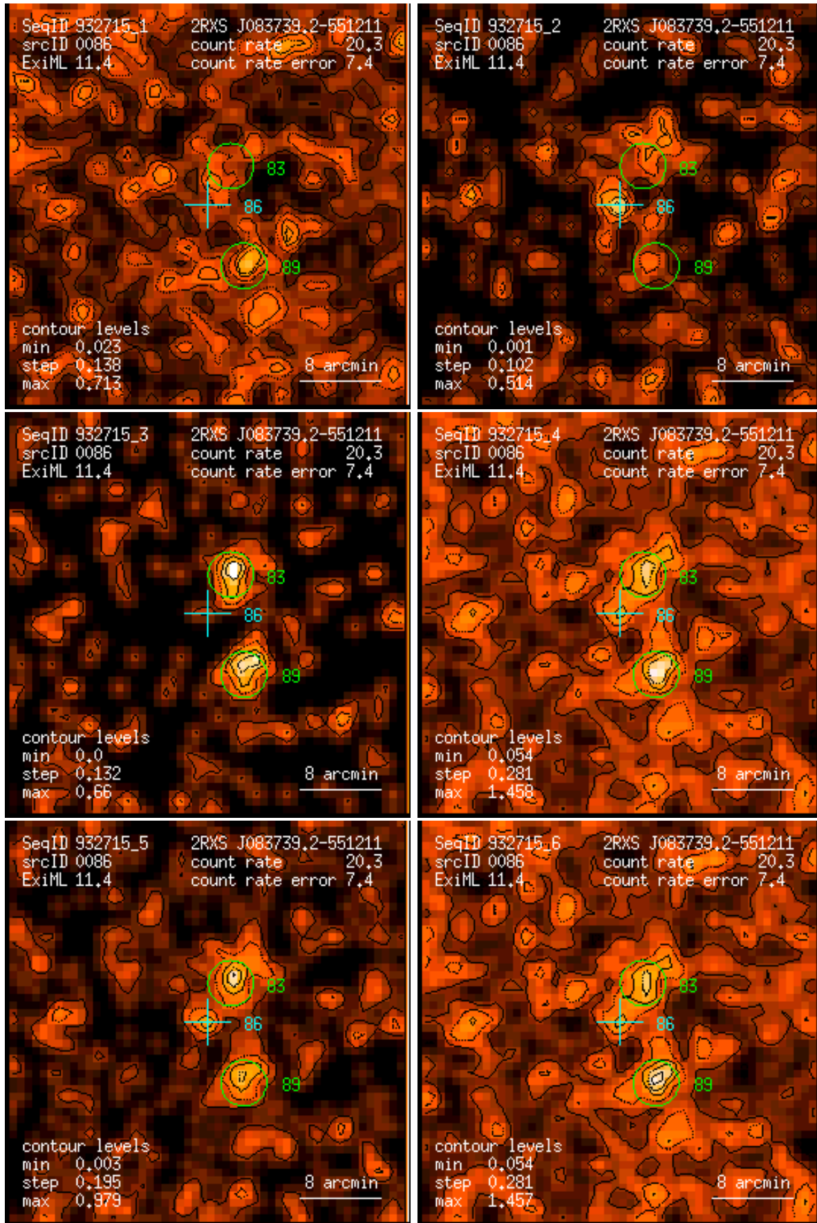
Figure 86: RASS 932715: detection 0086: band rate images, Gaussian filter: (1) PSPC channels 11 – 41, (2) 52 – 90, (3) 91 – 201, (4) 11 – 235, (5) 52 – 201, (6) 11 – 201. Broad band rates in counts/ks. Band rate contour levels in counts/ks/arcmin 2 .
