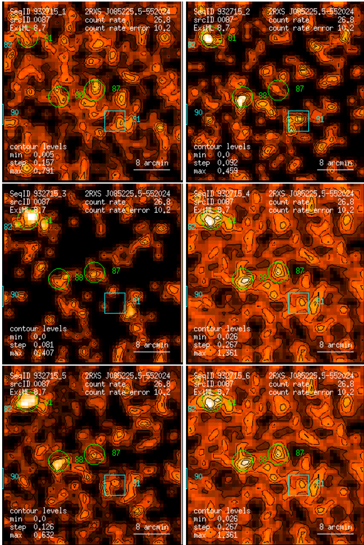
Figure 87: RASS 932715: detection 0087: band rate images, Gaussian filter: (1) PSPC channels 11 – 41, (2) 52 – 90, (3) 91 – 201, (4) 11 – 235, (5) 52 – 201, (6) 11 – 201. Broad band rates in counts/ks. Band rate contour levels in counts/ks/arcmin 2 .
